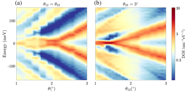
FIG. 3. (a) DOS as a function of twist angle for \theta_{12} = \theta_{23} . (b) DOS as a function \theta_{12} at \theta_{23} = 3^\circ , both on a logarithmic color scale.
