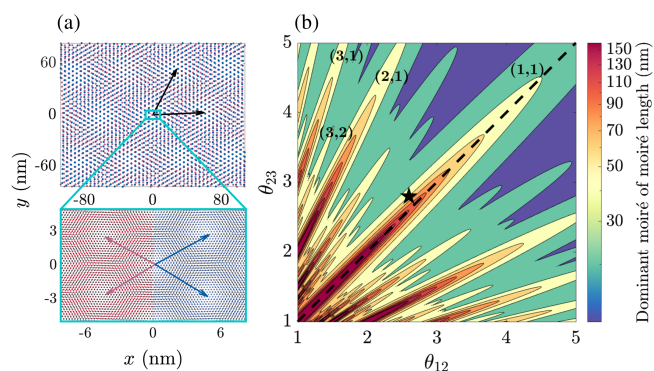
FIG. 1. Illustration of moiré of moiré pattern in tTLG for \theta_{12} = 2.6^\circ , \theta_{23} = 2.8^\circ . (a) Red and blue points represent the lattice points of the bilayer moiré supercells between L1-L2 and L2-L3, respectively. Black arrows represent dominant moiré of moiré supercell lattice vectors. A blowup of the small boxed area is shown below, with points representing monolayer lattice points, for L1 and L2 on the left half and for L2 and L3 on the right half. The moiré lattice vectors (red and blue arrows) are slightly rotated and have different lattice constants. (b) The dominant moiré of moiré length on a logarithmic color scale. The black star corresponds to the twist angle in (a), and (m, n) labels the dominant moiré of moiré harmonic in the nearby lobe. Black dashed line represents \theta_{12} = \theta_{23} .
