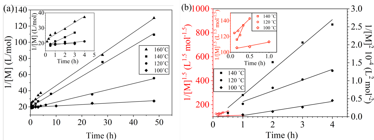
Figure 7. Linearized kinetic plot of (a) the DCDPS/BPA reaction and (b) the DFDPS/BPA reaction at conversions < 90% (hollow red markers) fit to a 2.5-order rate expression (red line), and at conversions > 90% (solid black markers) fit to a third-order rate expression (black line) at various temperatures with potassium carbonate as the base.
