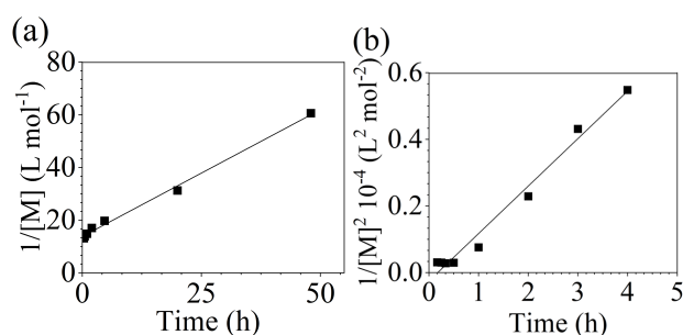
Figure 4. Linearized kinetic plots of: (a) second-order reaction for the polycondensation of DCDPS/BPA with Na_2CO_3 at 160 °C, and (b) third-order reaction for the polycondensation of DFDPS/BPA with Na_2CO_3 at 140 °C.
