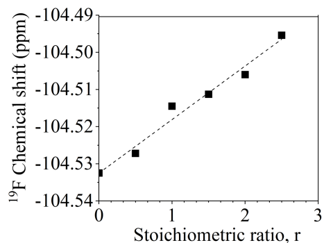
Figure 8. Chemical shifts of the ^{19}\text{F} nuclear magnetic resonance upon ArF interactions with \text{K}^+\text{PhO}^- at various stoichiometric ratios ( r , \text{K}^+\text{PhO}^-:\text{ArF} ).
