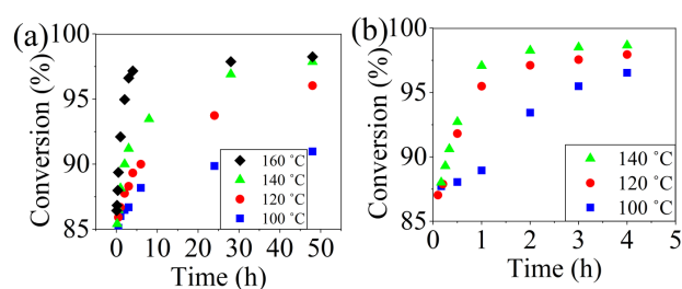
Figure 2. Plots of reaction conversion versus time for the polymerization of: (a) DCDPS and BPA, and (b) DFDPS and BPA at various temperatures with K_2CO_3 .
