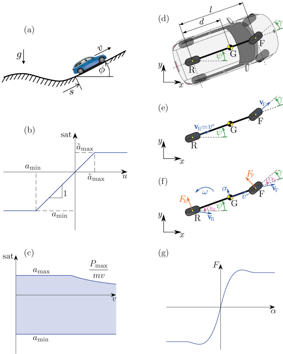
Figure 3. (a) Longitudinal model of an automobile with elevation. (b,c) Saturation functions used to model torque and power limitations. (d) Single-track lateral model of an automobile. (e) Kinematic bicycle model. (f) Dynamic bicycle model. (g) Lateral tyre force characteristics.
