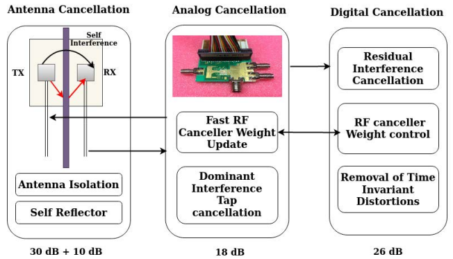
Figure 1: mmFD: Bidirectional full-duplex mm-Wave
