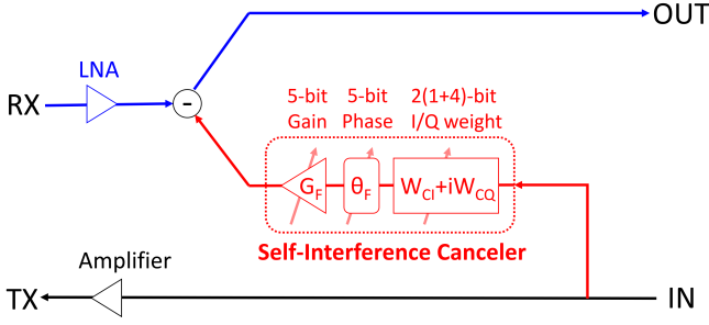
Figure 4: Simplified functional schematic of our chip
