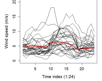
Fig. 3: Day-to-day variations at BROW on January 2008.
