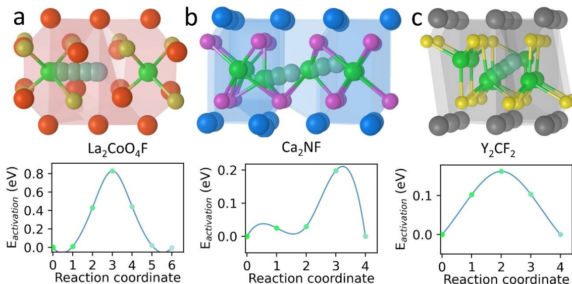
Figure 2: NEB study of F - diffusion kinetics. a. Vacancy diffusion in La 2 CoO 4 F. A tetrahedral F - moves to an adjacent vacant tetrahedral site in the LaO layer. The plot shows the diffusion barrier for the motion of F - . b. Interstitialcy mechanism in Ca 2 NF. A tetrahedral F - interstitial displaces an octahedral F - , which moves to a tetrahedral interstitial site on the opposite side as the original. c. Vacancy diffusion mechanism in Y 2 CF 2 . A tetrahedral F - moves to an adjacent tetrahedral site.
