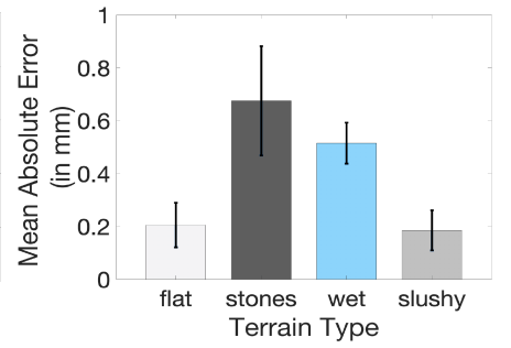
Figure 16: Tread Depth Error vs. Terrain Type
