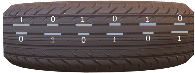
Figure 7: Osprey combats debris by laying Aluminium strips in the groove, which emulate a spatial code. Different grooves have different coded bit patterns encoded using pulse width modulation.
