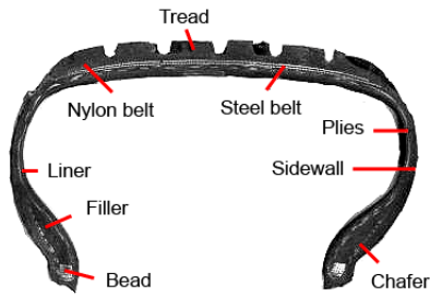
Figure 2: Depicts different components of a tire – distinct tread patterns, grooves running along the circumference, steel belts, nylon belts, etc. [50]
