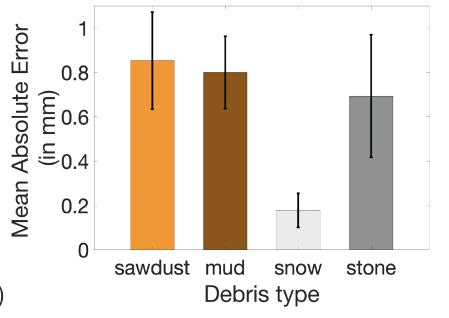
Figure 13: Tread Depth Error vs. Debris Type
