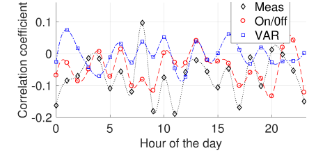
Fig. 13. Correlations between on time and the following off time.
