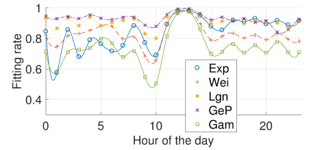
Fig. 7. On time fitting rates achieved by on/off models with different distributions.
