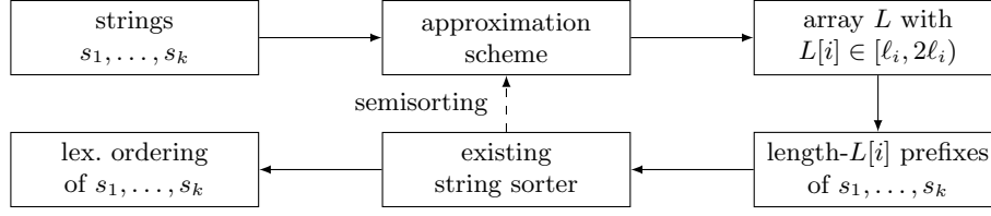
Fig. 2. Deriving D -aware string sorters from existing D -unaware solutions.
