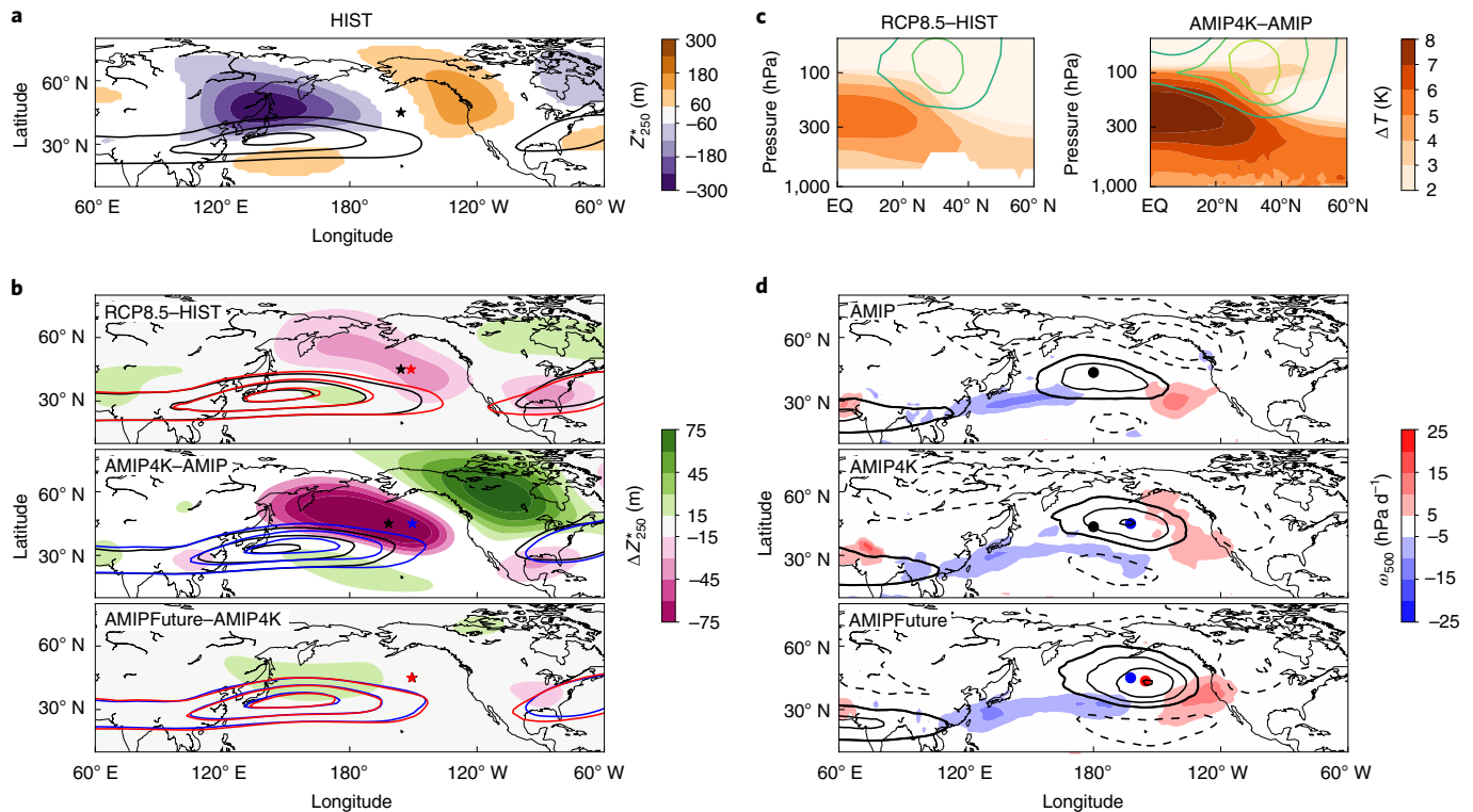
Fig. 4 | Eastward shift of the subtropical jet exit. a , Z'_{250} (shading) and \bar{U}'_{250} (contours at 35 \text{m s}^{-1} , 50 \text{m s}^{-1} and 65 \text{m s}^{-1} ) in HIST boreal winter. The node of Z'_{250} is indicated by the star. b , Responses of Z'_{250} (changes in shading and nodes denoted by star symbols) and \bar{U}'_{250} (contours) to anthropogenic warming in coupled models (top; from HIST in black to RCP8.5 in red), uniform warming (middle; from AMIP in black to AMIP4K in blue) and warming pattern (bottom; from AMIP4K in blue to AMIPFuture in red). c , Changes in the zonal-mean temperature (shading) and zonal wind (contours; 2.5 \text{m s}^{-1} interval) under anthropogenic warming (left; from HIST to RCP8.5) and forced by uniform surface warming (right; from AMIP to AMIP4K). d , MJO phase-3 teleconnection in simulations of AMIP, AMIP4K and AMIPFuture. The dots denote the Z'_{250} centres (black for AMIP, blue for AMIP4K and red for AMIPFuture).
