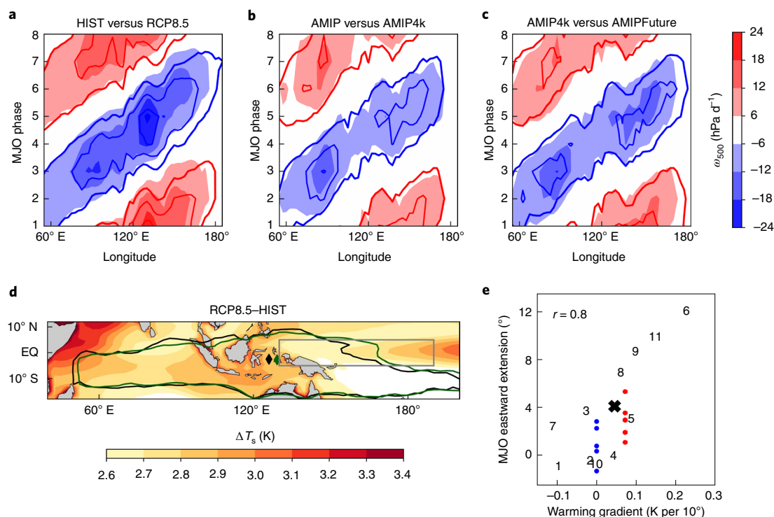
Fig. 3 | Eastward extension of the MJO itself. a , Anomalous \omega_{500} averaged over 10^{\circ}\text{S} – 10^{\circ}\text{N} as a function of the MJO phase and longitude in HIST (shading) and RCP8.5 (contours, with the same interval as in shading for HIST). b , Same as a but for AMIP (shading) and AMIP4K (contours). c , Same as a but for AMIP4K (shading) and AMIPFuture (contours). d , Surface warming pattern ( \Delta T_s ) projected under anthropogenic warming by the multi-model mean. The boundary (contour) and centroid (diamond symbol) of the active MJO region are denoted (black for HIST and green for RCP8.5). e , Intermodel scatterplot between the warming gradient (over the longitudes denoted by the grey box in d ) and the eastward MJO extension. Individual models are indexed and the cross symbol indicates the multi-model mean. The Pearson correlation coefficient r=0.8 . The blue and red dots denote the MJO extension in individual simulations of AMIP4K and AMIPFuture, respectively.
