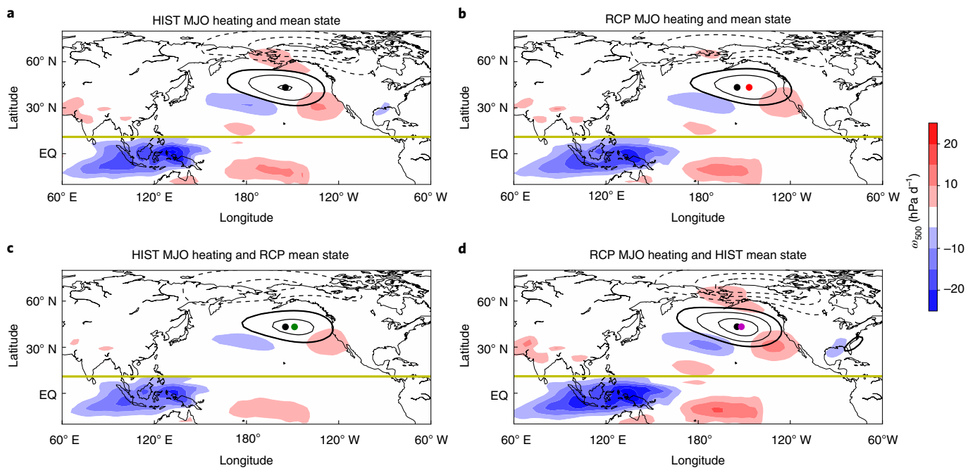
Fig. 2 | Responses of the MJO teleconnection to changes in MJO heating and large-scale mean state. a , Anomalous Z_{250} (contours at an interval of 12 m, solid for positive) and \omega_{500} (shading) associated with MJO phase 3 in LBM. Both MJO heating and mean state are from HIST. b , Same as a but with MJO heating and mean state both from RCP8.5. c , Same as a but with mean state from RCP8.5. d , Same as a but with MJO heating from RCP8.5. For a–d , the dot symbols denote the Z_{250} centre (black for a and colours for b–d ).
