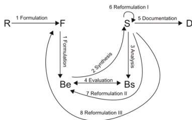
(a) (b) Figure 3. (a) FBS framework, (b) situated FBS framework (based on [15])
