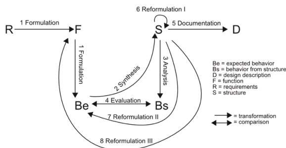
Figure 1. FBS framework (based on [14])
