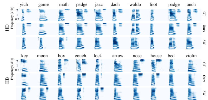
Fig. 6. Decoding results on each one of HD and HB testing set. GT and SW denote ground truth and SpecWaveNet, respectively.
