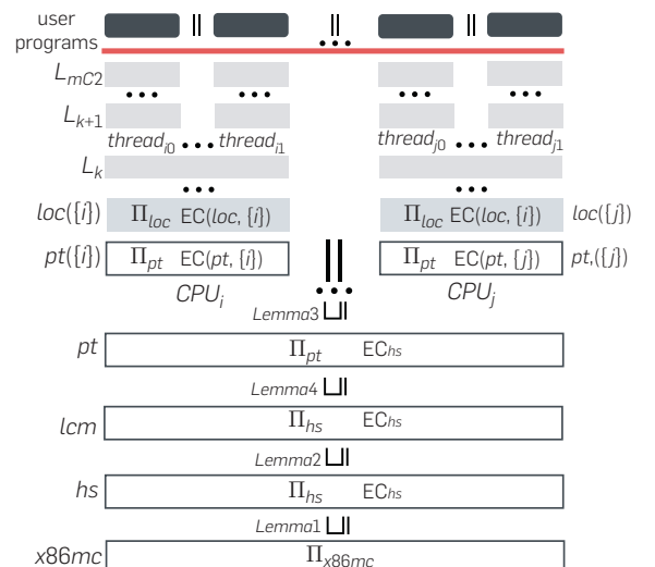
Figure 5. Contextual refinement between concurrent layer machines.
