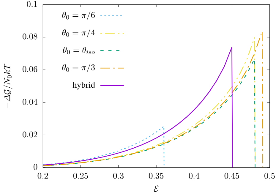
FIG. 7.5. Comparison of the DEA usable work of the hybrid network to the uniaxial networks with \sigma = 0 . While the most usable work can be derived from a uniaxial, \sigma = 0 network with properly chosen \theta_0 for a given \varepsilon , the hybrid network combines both stability and an enhanced usable work. In fact, the hybrid network performs \approx 75\% better than the isotropic network.
