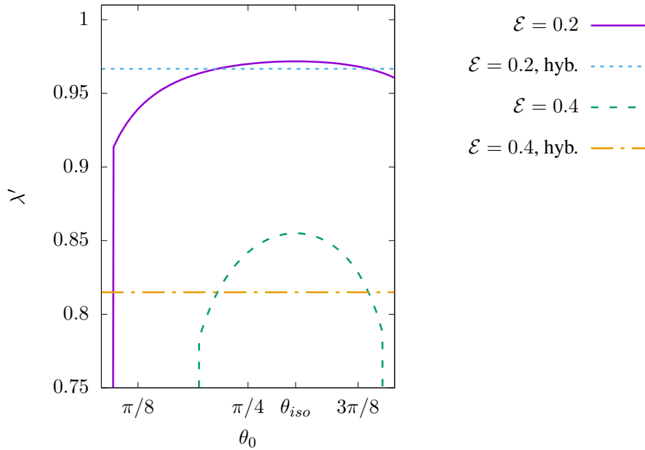
FIG. 7.3. Comparison of the DEA deformation of the hybrid network to the uniaxial networks with \sigma = 0 . The uniaxial networks have varying \theta_0 . Notice: for a given \mathcal{E} , the hybrid network deforms more than the uniaxial isotropic network (i.e. \theta_0 = \theta_{iso} ). However, for \mathcal{E} low enough, there is always some \theta_0, \sigma = 0 for which the uniaxial network has a large induced deformation than the hybrid network.
