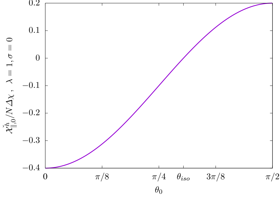
FIG. 5.3. Approximate \check{\chi}_{\parallel,0}^h for \sigma = 0 and \lambda = 1 . In this case, \check{\chi}_{\parallel,0}^h does not vanish and is \mathcal{O}(N) .
