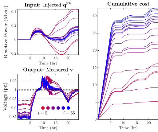
Figure 9. Stationary control with weak policy ( \theta_i \approx 0.01/m ). Unstable with deep PV penetration.
