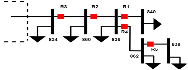
Fig. 2: Protective relays in a radial network
