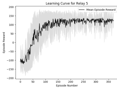
(a) Relay 5: Episodic reward
