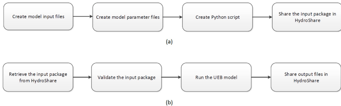
Fig. 6. The functionality of the added web services in HydroDS. Panel (a) for model input package preparation; Panel (b) for model simulation.
