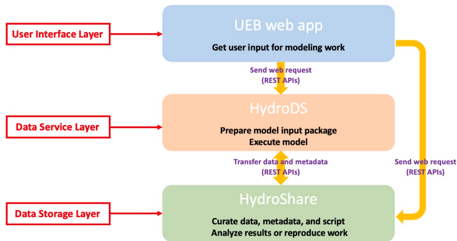
Fig. 1. A three-layer web service based architecture to integrate hydrologic data and modeling web services (e.g., HydroDS) with a data sharing system (e.g., HydroShare).
