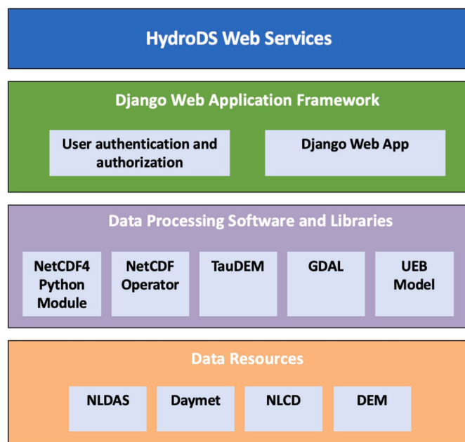
Fig. 2. The HydroDS system architecture.
