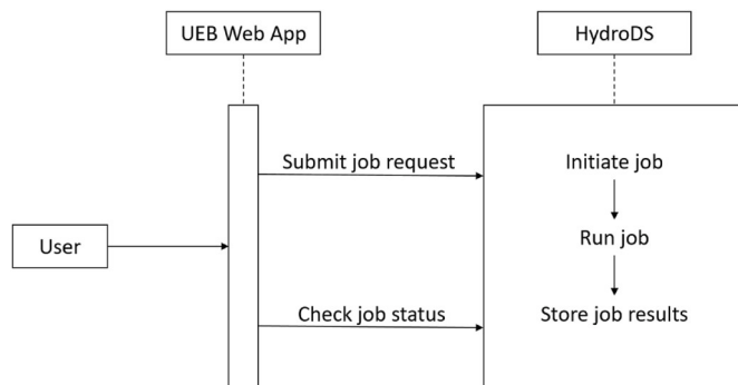
Fig. 7. Job management workflow.
