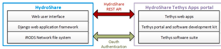
Fig. 3. System architecture of HydroShare and HydroShare Tethys Apps portal.
