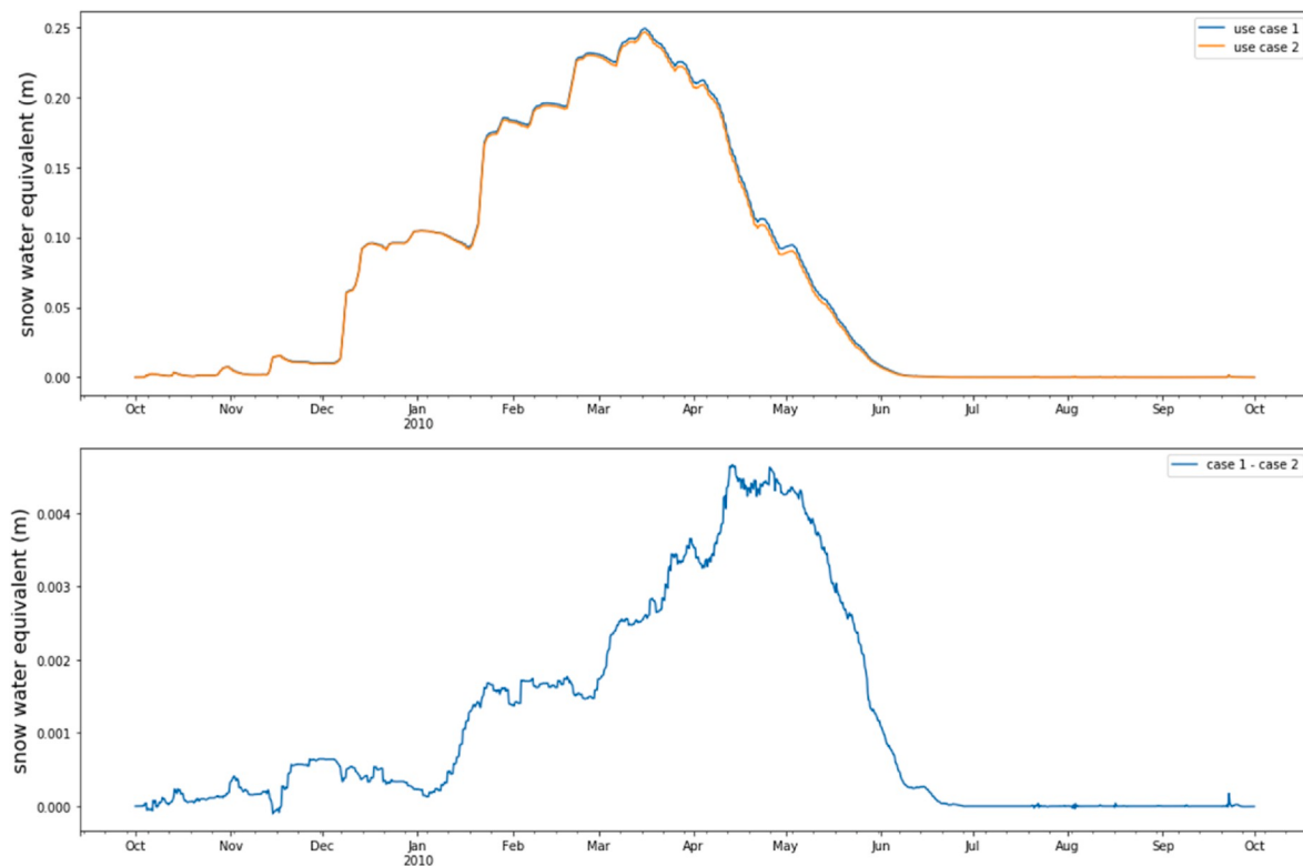
Fig. 13. Comparison of snow water equivalent created by the two uses cases.
