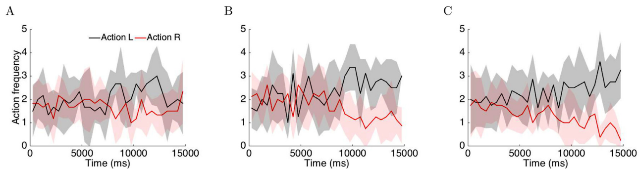
Fig. 9. Action frequencies when reward delivery is probabilistic. All panels represent the number of L (black) and R (red) actions performed across time (discretized each 50 ms) when action selection is rewarded with probability p_L = 0.65 (A), p_L = 0.75 (B), or p_L = 0.85 (C) with p_L + p_R = 1 . Traces represent the means over 8 different realizations, while the transparent regions depict standard deviations. (For interpretation of the references to colour in this figure legend, the reader is referred to the web version of this article.)
