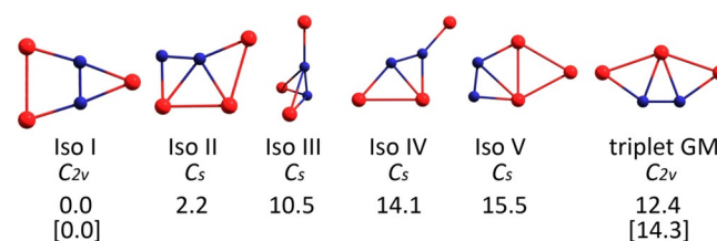
Figure 2. Five lowest energy singlet spin state isomers and one triplet spin state isomer of B _2 Al _3 ^- , their point group symmetries, and zero-point energy corrected relative energies (in kcal mol ^{-1} ) at the CCSD(T)/aug-cc-pwCVTZ and CAS(8,8) NEVPT2/aug-cc-pwCVTZ levels of theory [in square brackets]. The solid rods between atoms facilitate visualization, and do not necessarily represent bonds here and elsewhere. B is blue, Al is red.
