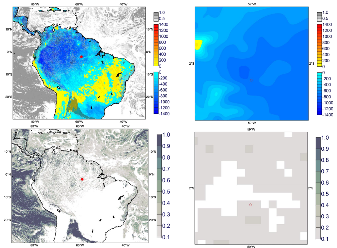
Figure 4. Top panel: IFS models results of the accumulated (from 15 to 18 UTC) net ecosystem exchange in units \text{g m}^{-2} \text{ day}^{-1} of the entire Amazonian basin (left) and zoom in to the simulated domain (right) (see Figure 2). Color bars: Negative and positive values represent a sink and a source of the net exchange ecosystem \text{CO}_2 , respectively. White-black bars represent the cloud cover ranging from 0 to 1. Bottom panel: IFS model results of low cloud cover (from 0 to 1) of the entire Amazonian basin (left) and a close-up of the simulated region (right). The variables correspond to 10 th September 2014. The circle marks the DALES domain and the K34 (T0k) site of the GoAmazon2014/15 experiment.
