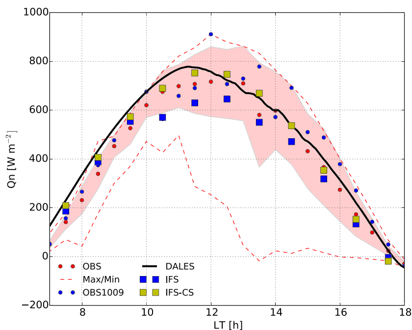
Figure 5. The observed and simulated available net radiation energy ( Q_n ). Observations (mean, standard deviation, and maximum and minimum) refer to the entire month of September 2014, collected during the GoAmazon2014/15 campaign. Observations were made above the canopy at the T0 Ksite. OBS1009 stands for the observations made on 10 September 2014. The DALES and IFS results are from 10 September 2014. IFS-CS represents the net available radiation under clear-sky conditions.
