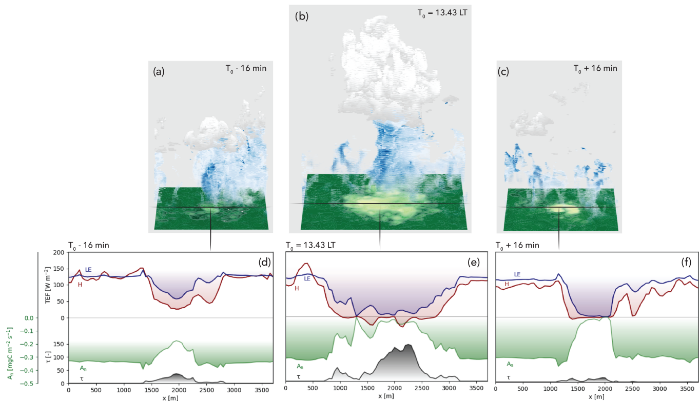
Figure 3. Top panel: three stages, around 13.43 LT (10 September), of a shallow cumulus cycle: (a) early formation, (b) maturity, and (c) dissipation. The x, y, and z axes are 4,000, 4,000, and 3,000 m, respectively. The blue color represents the specific humidity with maximum values of 5 \text{ g}_w \text{ kg}_a^{-1} . The green (more open stomata) to yellow (more close stomata) at the surface is the canopy of surface resistance, a representation of the stomatal aperture, with values ranging from 220 to 240 \text{ s m}^{-1} . Bottom panel: At the surface, the impact of the cloud disturbances (radiation, cold temperatures, and water vapor deficit) on the energy (H in red, TEf: turbulent energy fluxes), moisture (LE in blue), and CO 2 assimilation ( A_n in green) fluxes are shown at (d)–(f). Cloud thickness (gray) is quantified by the cloud optical depth ( \tau ). The color shading is to improve the visualization.
