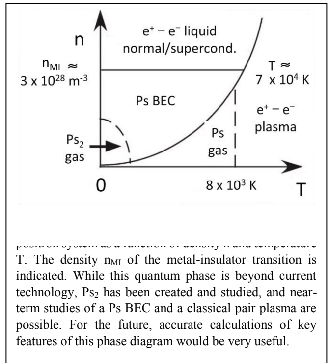
Fig. 1 [2]. Most of the phases have yet to be created and studied. An exception is that, using a specially tailored pulsed positron beam, sufficiently dense gases of positronium atoms have been created at the surface of a solid to conduct the first studies of the Ps molecule, \text{Ps}_2 ( e^+e^-e^+ ) [6]. Efforts are underway, using advanced versions of this technology to create a Bose-condensed gas (BEC) of Ps atoms in cavities close to the surface of a solid [7]. Experiments are also in progress to create a classical pair plasma in a levitated, superconducting magnetic dipole trap [8].
