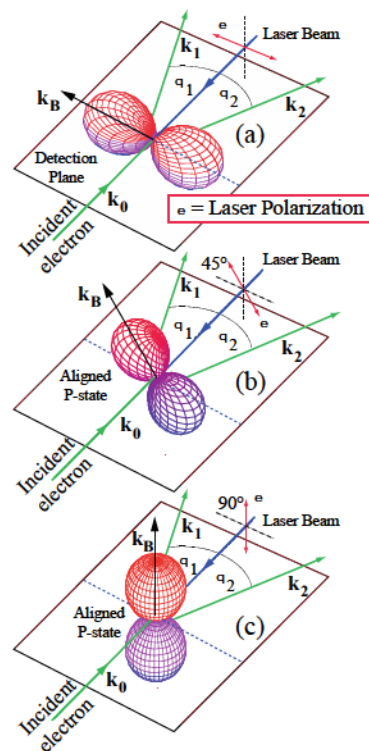
Figure 1 – Alignment of the excited P-state with respect to the detection plane spanned by \mathbf{k}_1 and \mathbf{k}_2 . Three examples are shown, with the state aligned in the plane, at 45^\circ to the plane and orthogonal to the plane.
