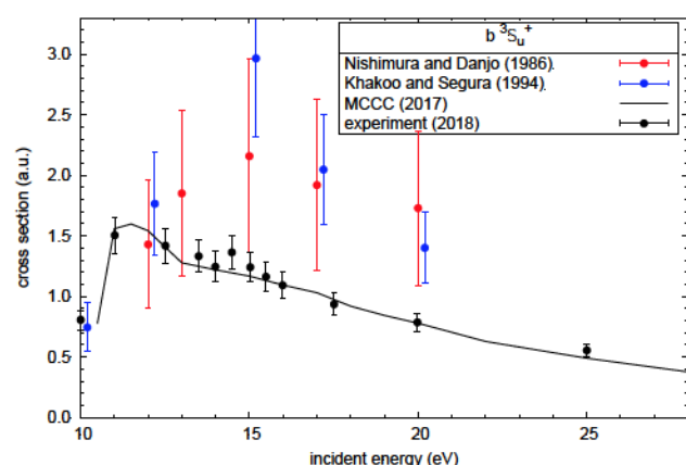
Figure 2: e\text{-H}_2 b^3\Sigma_u^+ excitation see Ref.[8] for details.
