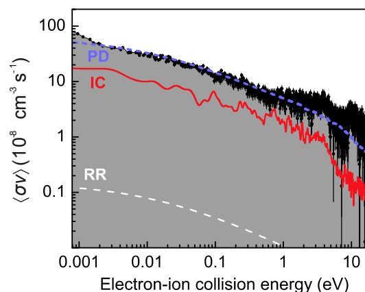
Figure 1 – Dielectronic recombination cross-section of W^{18+} ions ( 4f^{10} valence configuration) measured with the storage-ring merged-beams method. (Cross section \sigma multiplied with the collision velocity v and convolved with the electron energy spread.) Calculations show radiative recombination (RR), dielectronic recombination by one-electron promotion in intermediate coupling (IC), and a model including statistical partitioning and a damping correction (PD). (Adapted from Ref. [3]. Beam-merging artefacts at <0.001 eV are negligible in the plasma rate constants.)
