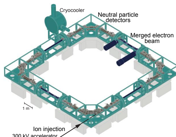
Figure 2 – The cryogenic electrostatic storage ring CSR that started operation in 2015 with the recently added electron beam section. The elements enclosing and steering the ion beam, the electron collision region and the particle detectors are operated below 10 K. (Adapted from Ref. [6].)
