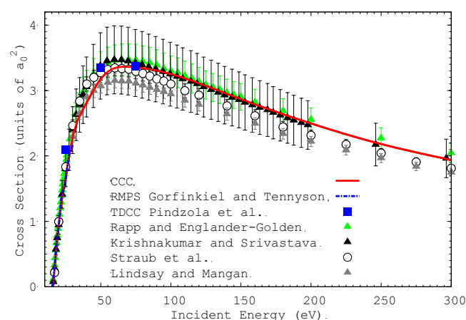
Figure 1: e-H 2 total ionization, see Ref.[7] for details.
