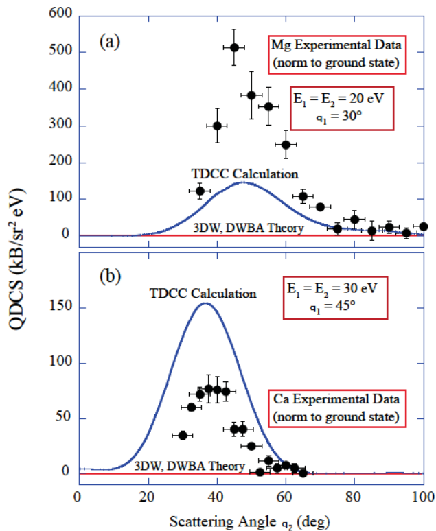
Figure 2 – QDCS when \mathbf{k}_B is aligned orthogonal to the plane for (a) Mg and (b) Ca. Both 3DW and DWBA theories predict QDCS = 0 for all scattering angles. The TDCC calculation which includes un-natural parity states predicts a non-zero cross section, although the magnitudes do not agree with experiment. The data are normalized to results for ground state ionization.
