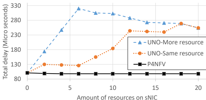
Fig. 8: Comparison of observed delay of P4NFV Vs. UNO [7]
