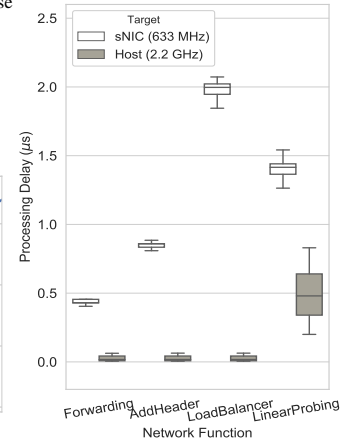
Fig. 4: NF Processing delay
