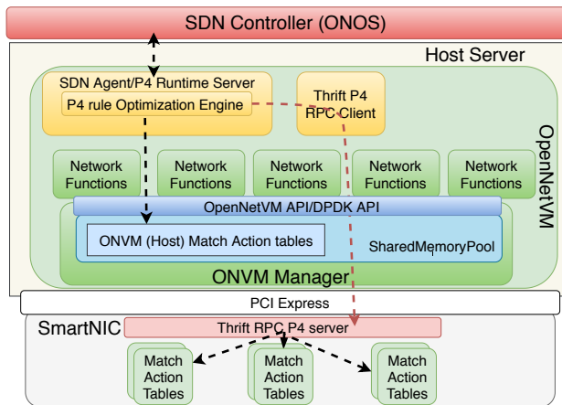
Fig. 1: P4NFV Architecture
