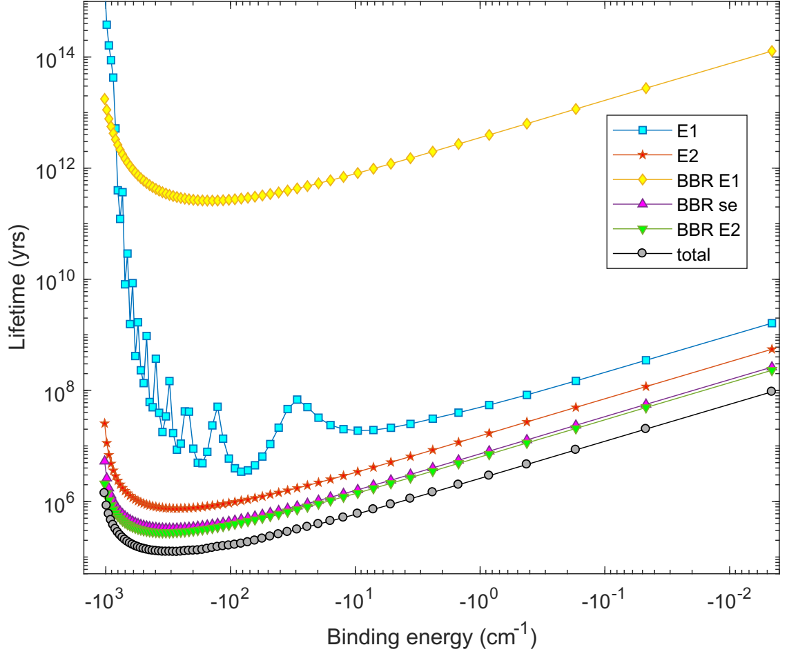
FIG. S3: Overall lifetimes of the X0_g^+ ( J=0, v ) states along with the individual contributions. The v ranges from 0 to 62, left to right.
