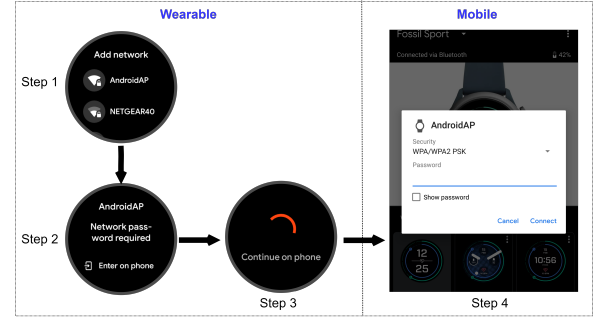
Figure 2: Example of the inter-device communication between a wearable and a mobile device. The setup of a WiFi connection starts in the wearable, but then the process continues on the mobile due to the difficulty of typing the password on the wearable device.
