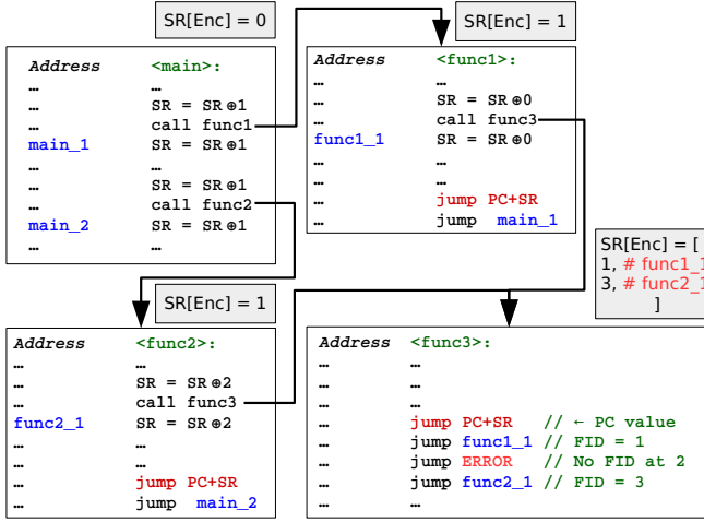
Fig. 9. Illustration \mu RAI's relative-jump TLR policy.
