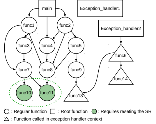
Fig. 8. Conceptual illustration of \mu RAI's call graph analysis.
