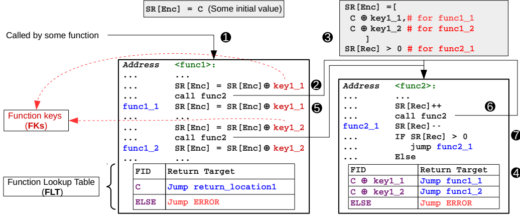
Fig. 5. Illustration of \mu RAI's design. Enc: Encoded SR. Rec: Recursive SR.
