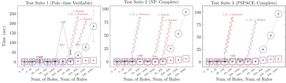
Fig. 10: Mohawk inputs [4] converted to ATRBAC-safety instances using one time-slot. Test Suite 1 are inputs with non-negated preconditions only. Test Suite 2 are inputs with no revoke rules. Test Suite 3 are both positive and negated preconditions, and assign/revoke rules. Red wavy lines are tools that crashed/timedout during testing for certain input sizes.
