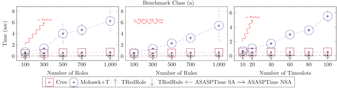
Fig. 8: Results on all tools for Benchmark Class (a). It comprises random input instances from a generator from Uzun et al. [2]. The curves interpolate averages, and the error-bars show the standard deviation.
