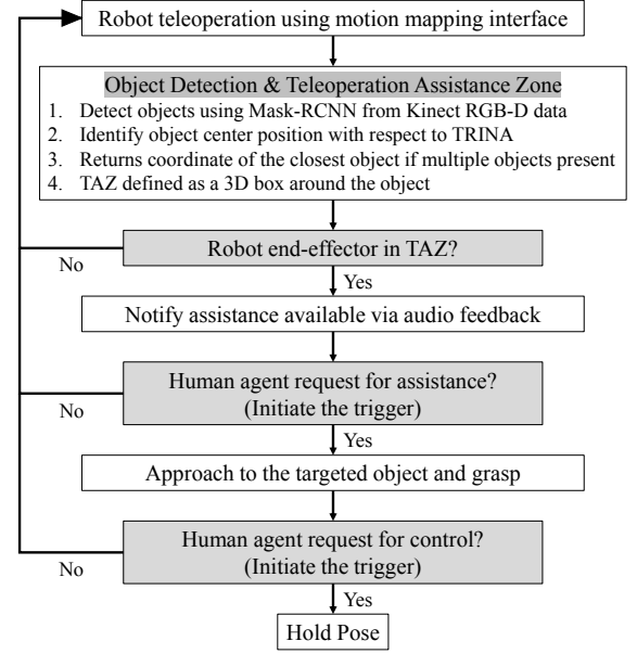
Fig. 3: Autonomous Grasping Function for Teleoperation Assistance.
