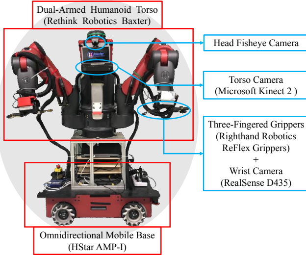
Fig. 2: Tele-robotic Intelligent Nursing Assistant (TRINA) system.
