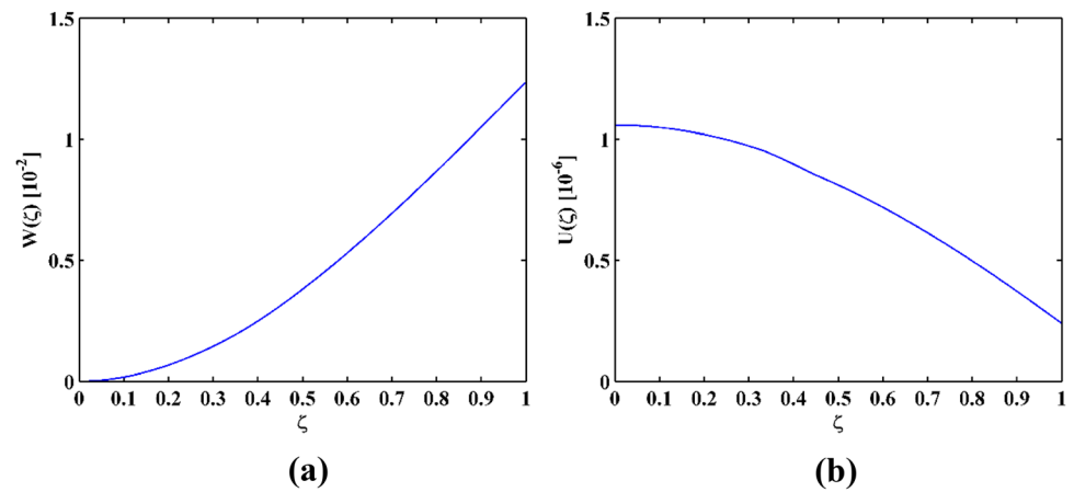
Fig. 11 Noisy a flexural and b longitudinal SRSHEs at excitation frequencies that are half of the flexural and longitudinal fundamental natural frequencies, respectively
