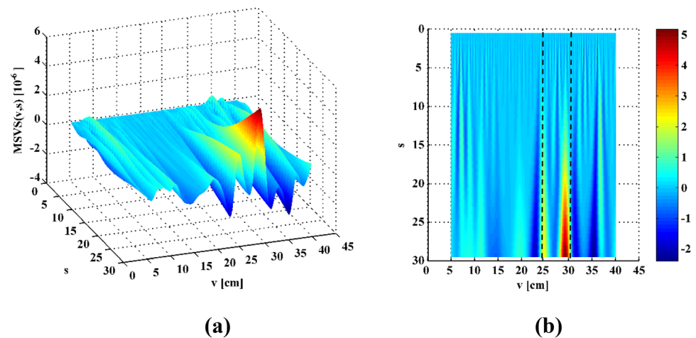
Fig. 20 a MSVS for the longitudinal SRSHE at 4900 Hz and b its top view
