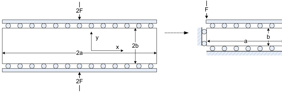
Fig. 2. The physical domain (left) and computational domain (right) of the Mandel's problem [18].
