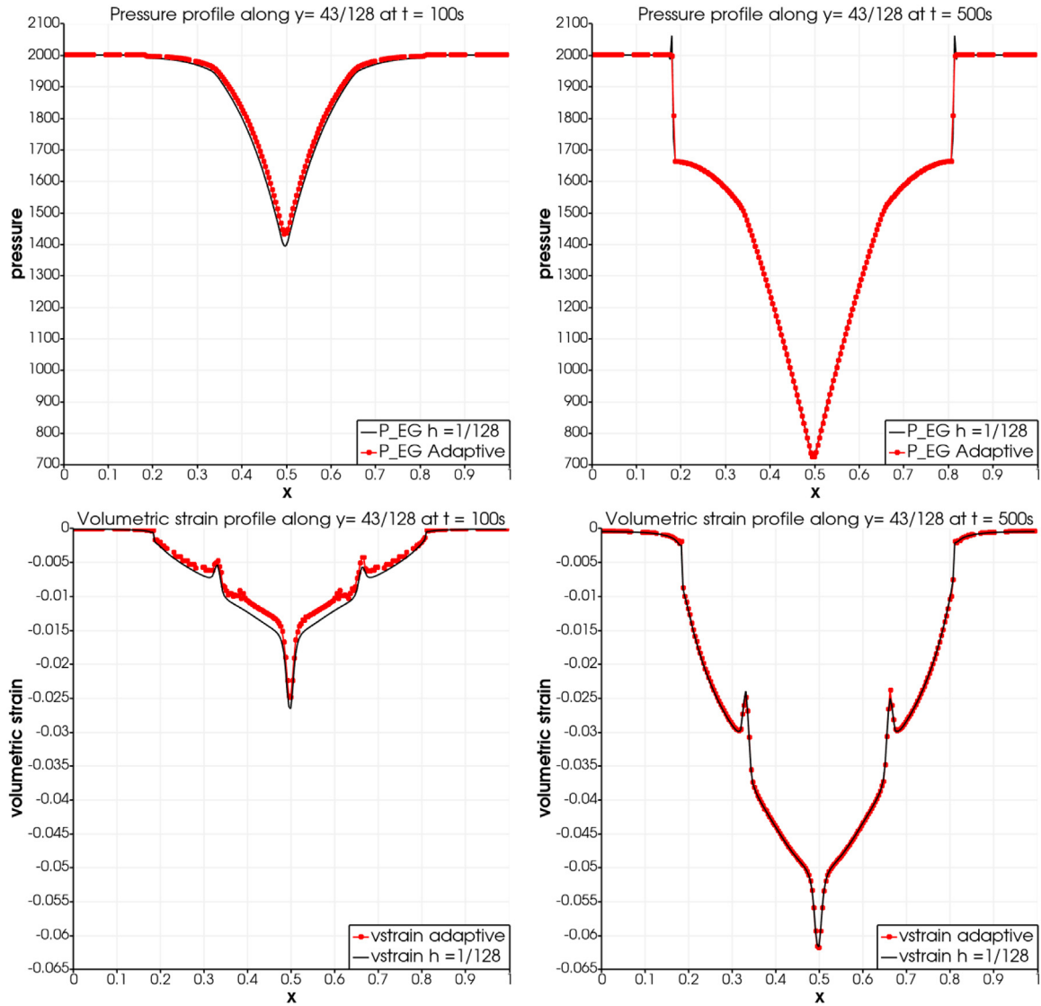
Fig. 5. Comparison of the solutions on the dynamic adaptive mesh and on a uniform fine mesh 128 \times 128 along y = 43/128 : top: pressure, bottom: volumetric strain; left: t = 100 s, right: t = 500 s.
