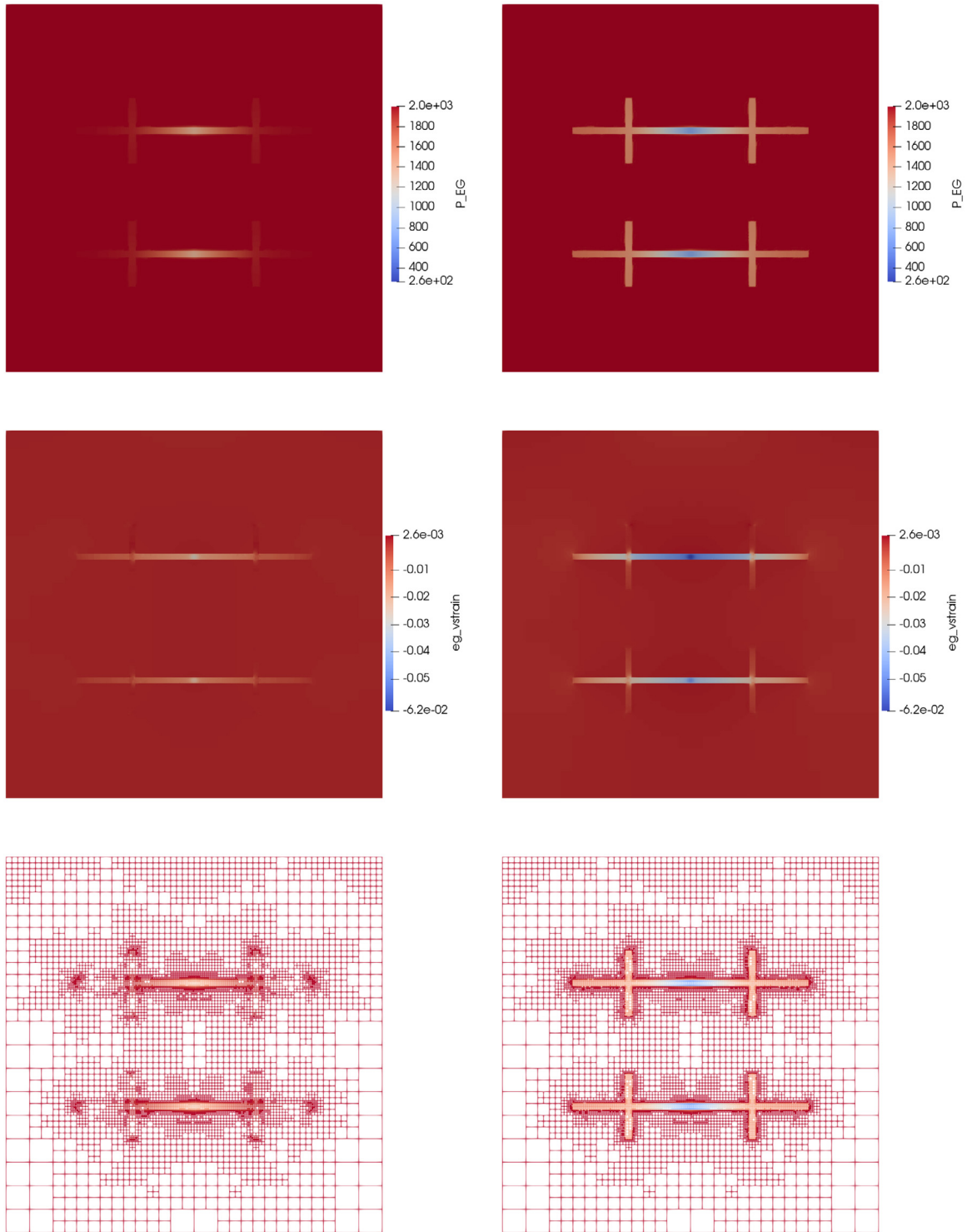
Fig. 4. Dynamic mesh adaptivity guided by the a posteriori error indicators: top: pressure, middle: volumetric strain, bottom: adaptive mesh; left: t = 100 s, right: t = 500 s.
