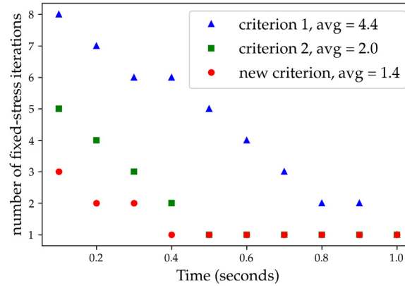
Fig. 6. Comparison of the number of fixed-stress iterations for each time step using difference stopping criteria for the Mandel problem.
