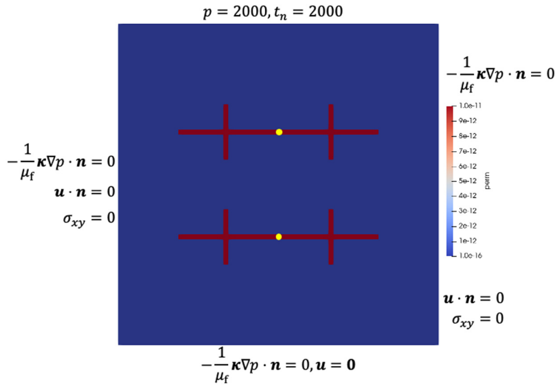
Fig. 3. Permeability field and model boundary conditions of the prototype unconventional reservoir model.
