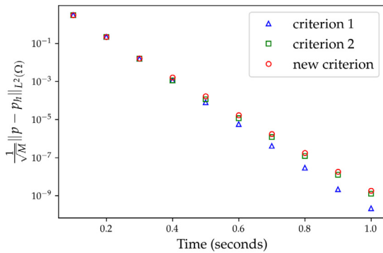
(a) Pressure solution errors comparison
