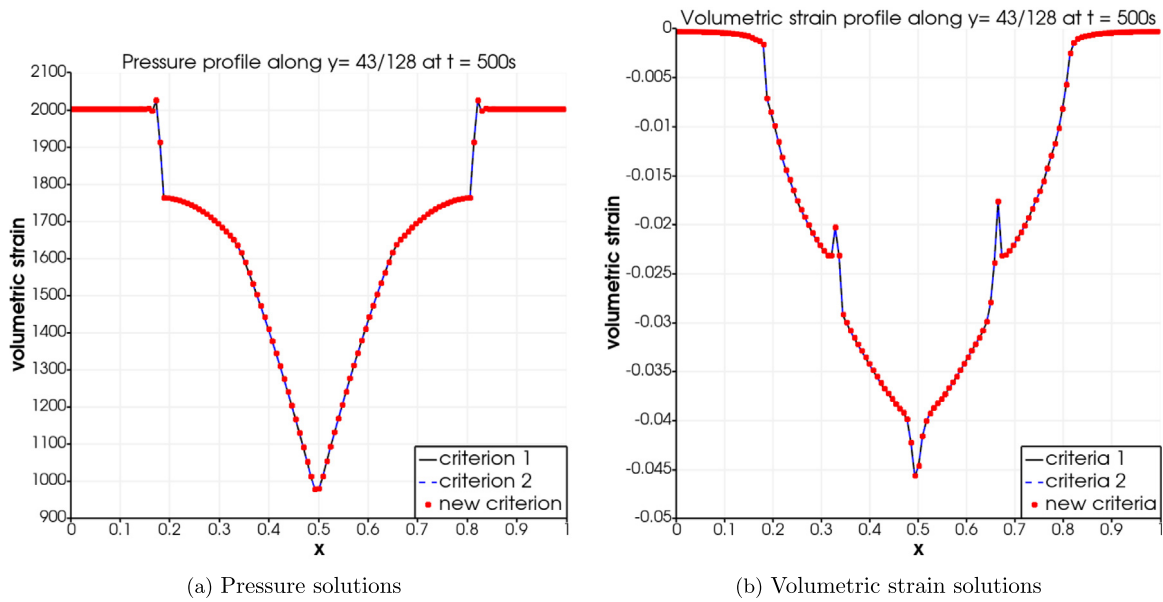
Fig. 8. Comparison of pressure and solutions at t = 500 s using different stopping criteria for the unconventional reservoir model.
