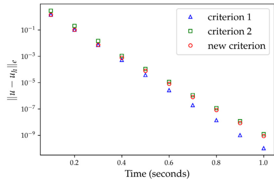
(b) Displacement solution errors comparison
