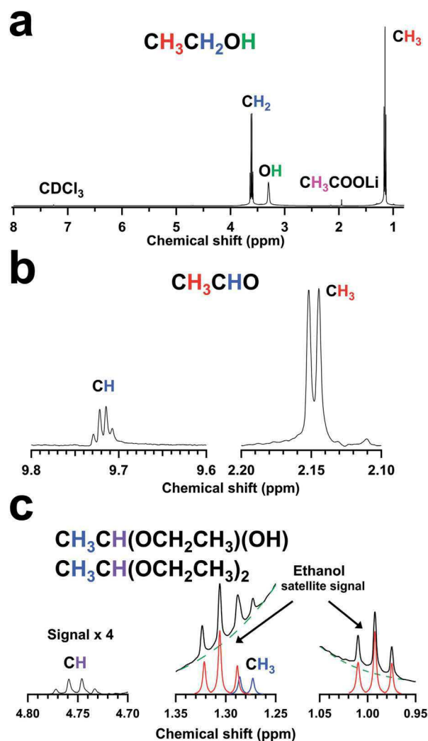
Fig. 6 NMR spectra of the reaction solution under synthesis condition with 4 : 1 reactants ratio of Li(OAc) : \text{Ce}(\text{NO}_3)_3 indicated the presence of (a) ethanol and lithium acetate, (b) acetaldehyde and (c) 1-ethoxyethan-1-ol and 1,1-diethoxyethane.
