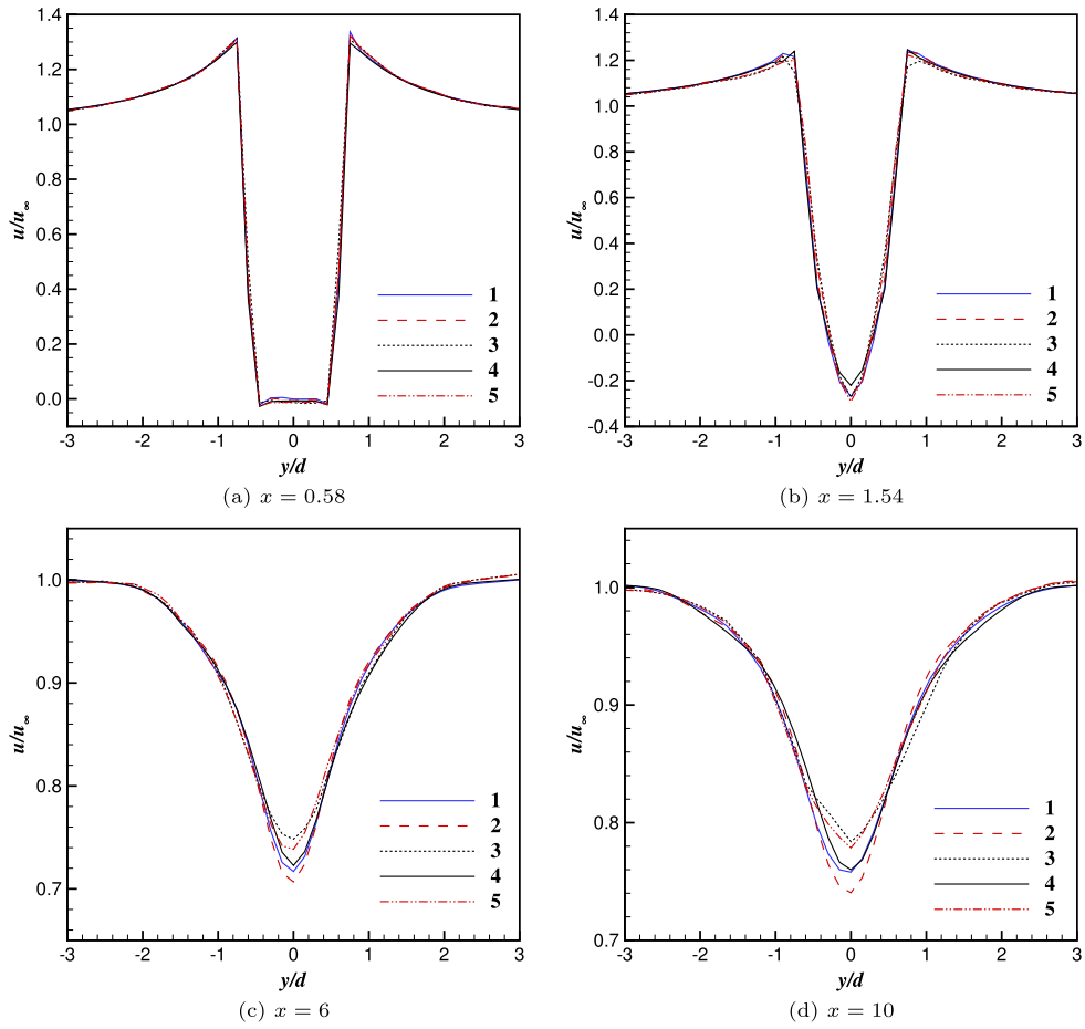
Fig. 9. Profiles of velocity component u in x -direction at different locations. Legend 1, p -uniform p^2 FR; Legend 2, p -adaptive p^2 FR with (v_{\max}, v_{\min}) = (0.1, 0.001) ; Legend 3, p -adaptive p^2 FR with (v_{\max}, v_{\min}) = (0.1, 0.01) ; Legend 4, p -uniform p^3 FR; Legend 5, p -adaptive p^3 FR with (v_{\max}, v_{\min}) = (0.1, 0.01) .
