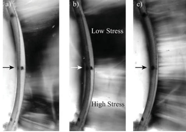
FIGURE 5. Flow-induced birefringence snapshots corresponding to the sequence of fluid rupture in the wake of the flexible sheet for a velocity of U = 10 mm/s. In (a), an FIB image is shown at the onset of sheet recoil, time t = 0 , in (b), t = 0.25 s, while in (c), t = 0.60 s which corresponds to the end of the recoil phase in the oscillation cycle. The bright regions highlight areas of large micelle deformation and large elastic stresses in the fluid while the darker regions show the locations where the micelles have broken down and the elastic stress in the fluid has been lost.
