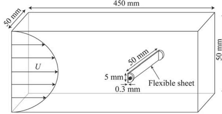
FIGURE 1. Schematic diagram of the setup.
