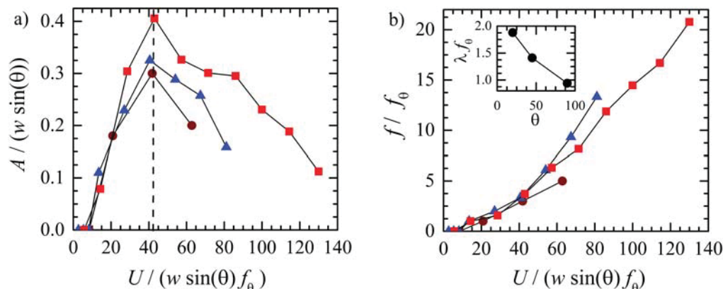
FIGURE 8. The dimensionless (a) amplitude and (b) frequency of oscillations as a function of the dimensionless flow velocity for flexible sheet inclination angles of 20^\circ (●), 45^\circ (▲) and 90^\circ (■). The inset in (b) contains the dimensionless product, \lambda f_\theta , as a function of inclination angle.
