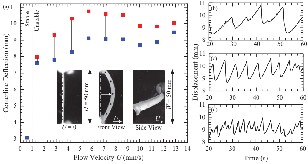
FIGURE 2. (a) The centerline deflection of the flexible sheet versus flow velocity, and the time histories of the centerline deflection of the sheet at (b) U = 4.3 mm/s, (c) U = 7.15 mm/s, and (d) U = 11.44 mm/s. The critical onset condition, U = 1.4 mm/s, corresponds to Wi_{crit} = 13 .
