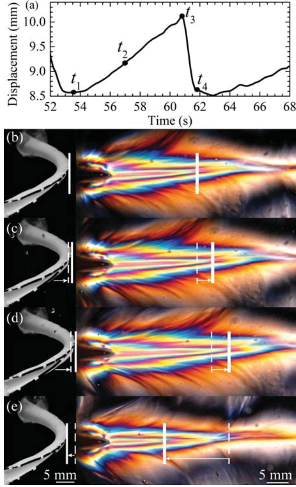
FIGURE 3. (a) Time history of the centerline deflection of the sheet for one period of oscillation, together with bright field images of deformed sheet (left), and the extensional birefringent patterns (right) at U = 4.3 mm/s and for (b) t_1 = 0 , (c) t_2 = 3.45 s, (d) t_3 = 7.2 s, and (e) t_4 = 7.95 s. The dashed lines highlight the change in the birefringence patterns and deformations of the sheet between each time interval. The FIB images are viewed perpendicular to the flow direction while the real bright field images are taken from an angle to the flow direction in order to show the entire length of the flexible sheet.
