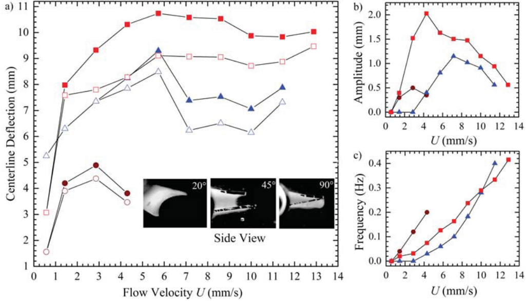
FIGURE 6. (a) Centerline displacement of the flexible sheet for 20°(●), 45°(▲) and 90°(■) inclinations. The filled and hollow symbols are used for the maximum and minimum flexible sheet displacements respectively during oscillations at each flow velocity. The inset contains the side views of the cross-flow deformation of the flexible sheet. (b, c) Amplitude and frequency of oscillations of the flexible sheet over the range of flow velocities tested. The error margin for the amplitude of oscillations is less than 10% for flow velocities below 4mm/s and less than 5% for higher flow velocities. The error margin is less than 5% for the frequency plots.
