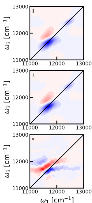
Figure 2. 2DES spectra for LH2 at waiting time zero for parallel (||, top), perpendicular (⊥, middle), and cross (x, bottom) polarization. Contour lines as plotted at 10% levels of the maximum of the individual 2DES spectrum. Red contours represent the absorption signal, while blue contours represent bleach.
