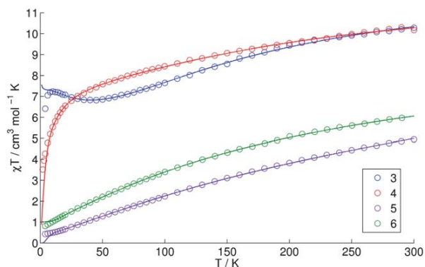
Fig. 3 \chi_{\text{M}}T vs. T data (circles) and fits (lines) for compounds 3–6. See Table 2 for fit parameters.
