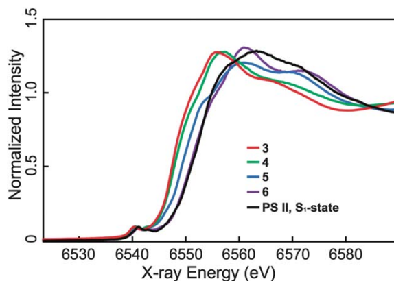
Fig. 2 Normalized Mn K-edge XANES spectra from complexes 3–6 compared with the spectrum from spinach PSII in the S 1 -state.
