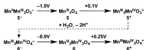
Scheme 2 Effect of oxidation state and oxido ligand content on leveling of reduction potentials for 5 and 6 .
