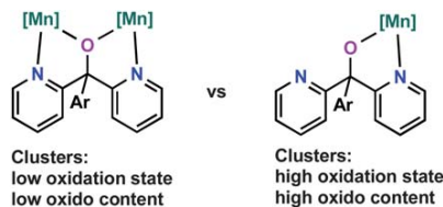
Fig. 6 Ligand flexibility as function of cluster oxido content and oxidation state: binding modes of dipyriddyalkoxide arms in clusters 1–7.
