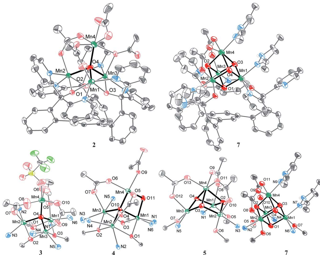
Fig. 1 Solid-state structures of complexes 2–5 and 7 . Top: depictions of full molecules 2 and 7 ; bottom: truncated \text{Mn}_4\text{O}_x cores. Thermal ellipsoids are drawn at 50% probability. Hydrogen atoms, outersphere anions, and solvent molecules are not shown for clarity. Bolded bonds highlight the \text{Mn}_4\text{O}_x cores. See ESI† for detailed crystallographic information. The structure of complex 5 has been reported previously. 33
