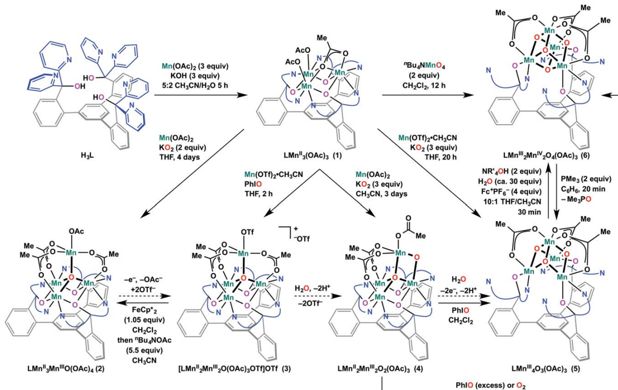
Scheme 1 Synthesis and interconversion of tetramanganese complexes 2–6 . Dashed arrows represent conceptual conversions involving water, proton and electron transfers. Curved lines represent 2-pyridyl groups. OAc = acetate. OTf = trifluoromethanesulfonate. \text{Fc}^+ = ferrocenium.
