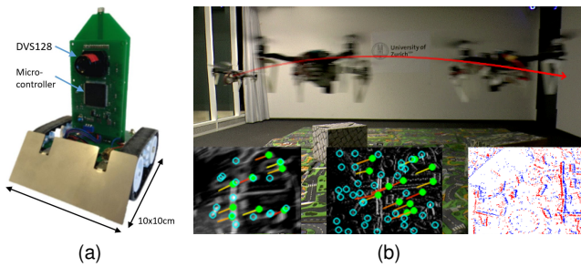
Figure 13. (a) Embedded DVS128 on Pushbot as standalone closed-loop perception-computation-action system, used in navigation and obstacle-avoidance tasks [240]. (b) Drone with a down-looking DAVIS, used for autonomous flight [27]. The high speed and dynamic range of events are leveraged to operate in difficult illumination conditions. The same visual-inertial odometry algorithm [27] is also demonstrated on high-speed scenarios, such as an event camera spinning tied to a rope.
