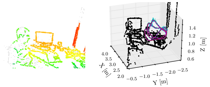
(a) Events & projected map. (b) Camera trajectory & 3D map.
