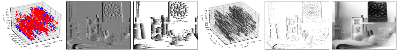
Figure 3. Several event representations (Section 3.1) of the slider_depth sequence [81]. From left to right: events in space time, colored according to polarity (positive in blue, negative in red). Event frame (brightness increment image \Delta L(\mathbf{x}) ). Time surface with last timestamp per pixel (darker pixels indicate recent time), only for negative events. Interpolated voxel-grid ( 240 \times 180 \times 10 voxels), colored according to polarity, from dark (negative) to bright (positive). Motion-compensated event image [82] (sharp edges obtained by event accumulation are darker than pixels with no events, in white). Reconstructed intensity image by [8]. Grid-like representations are compatible with conventional computer vision methods [83].
