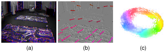
Figure 6. Two optical flow estimation examples. (a) and (b): indoor flying scene [175]. In (a), events (polarity shown in red/blue) are overlaid on a grayscale frame from a DAVIS. (b) shows the sparse optical flow (colored according to magnitude and direction) computed using [166] on brightness increment images. (c) A different scene: dense optical flow of a fidget spinner spinning at 750^\circ/\text{s} in a dark environment [103]. Events enable the estimation of optical flow in challenging scenarios.
