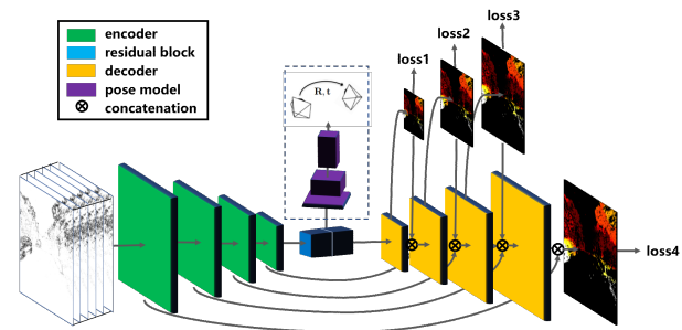
Figure 4. Events in a space-time volume are converted into an interpolated voxel grid (left) that is fed to a DNN to compute optical flow and ego-motion in an unsupervised manner [103]. Thus, modern tensor-based DNN architectures are re-utilized using novel loss functions (e.g., motion compensation) adapted to event data.
