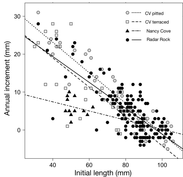
Fig. 8. Annual increment in shell length (mm) relative to initial shell length (mm) of Scutellastra laticostata . See Table S5 for regression equations
