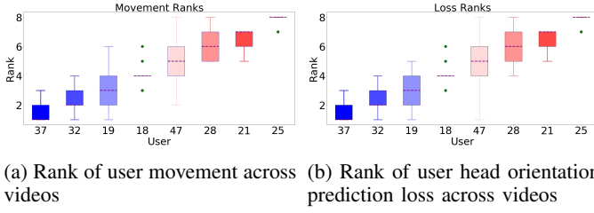
Fig. 6: Rank of user movement and prediction loss (compared to their peers) across videos (dataset 2, experiment 1). Users tend to be consistent across videos, both in terms of user movement and prediction loss.
