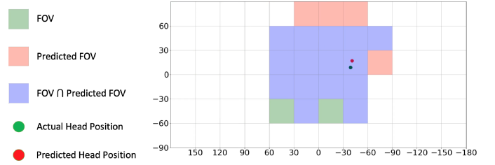
Fig. 1: Example relationship between a user’s actual FoV, and the user’s predicted Fov, with tiling. The user’s FoV is projected from the sphere onto a 2D plane, resulting in the irregular shapes shown above in the figure.
