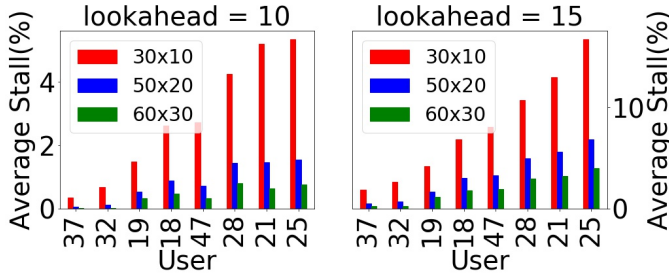
Fig. 11: Average stalls of selected users (dataset 2, exp. 1).
