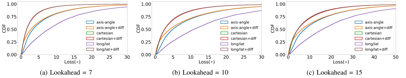
Fig. 3: CDF of prediction loss for different head orientation representations and lookaheads values. Cartesian coordinates plus time differencing has the lowest prediction loss.
