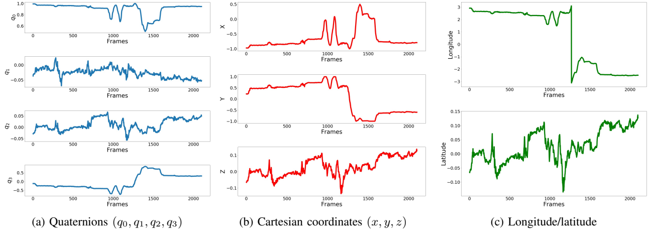
Fig. 2: Examples of different representations of the same head orientation trace. The same trace looks quite different under different representations, which can then affect the prediction method.
