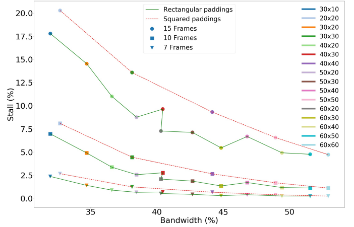
Fig. 9: Tradeoff between bandwidth usage and stalls, for different padding shapes and lookaheads. Rectangular paddings are at the frontier of the region, i.e. , they are Pareto-efficient.
