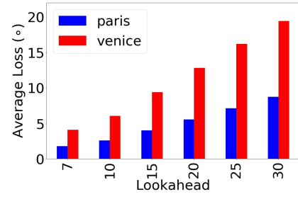
Fig. 12: Prediction loss is lower for the “Paris” video due to audio narration biasing the users’ FoVs towards a common region in the video (dataset 1).
