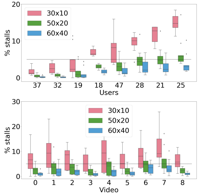
Fig. 14: Per-video vs. per-user customization
