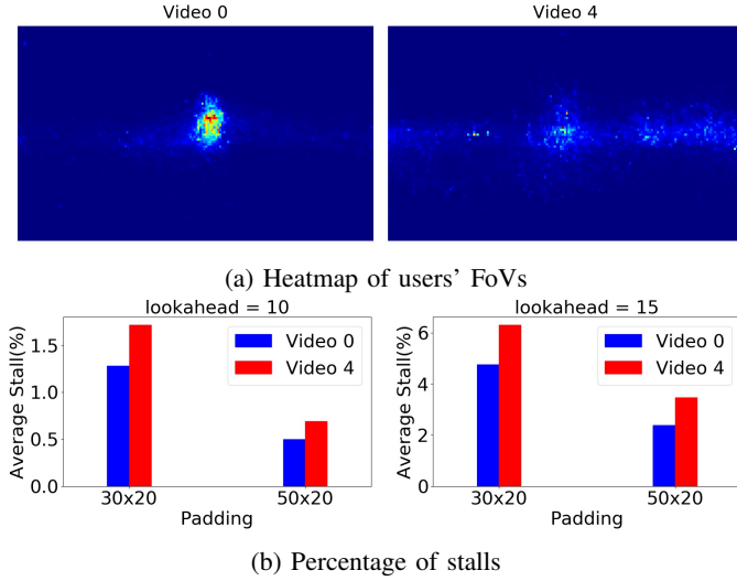
Fig. 13: User viewing behavior and stall probability for two videos. Video 0 has more concentrated user viewing patterns, and hence experiences fewer stalls, for different lookahead and padding sizes.
