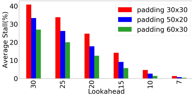
Fig. 10: Dependency between lookahead and stalls for different padding sizes (dataset 1).
