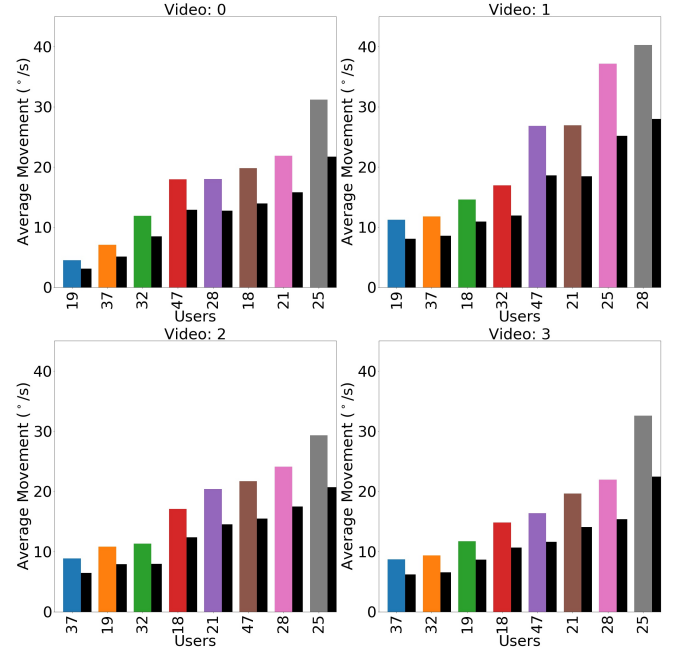
Fig. 5: Users' average head movement (colorful bars) is correlated with their prediction loss (black bars).
