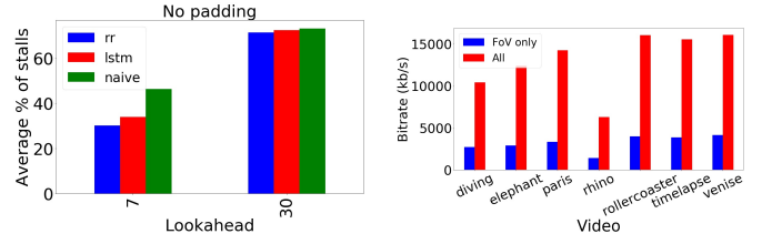
(a) % of stalls across all datasets, without padding (b) Bandwidth savings of perfect prediction vs. sending all tiles, for select videos (dataset 1)
