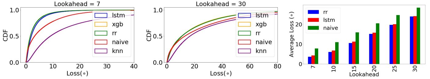
(a) Comparison of user prediction algorithms (lookahead L = 7 ).
