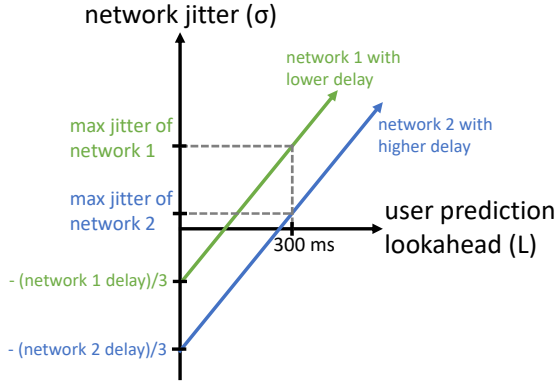
Fig. 15: Relationship between network delay, jitter, and prediction lookahead.
