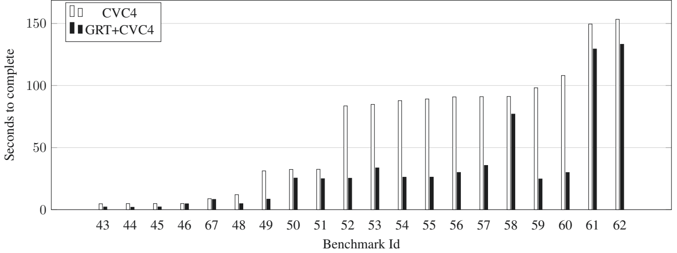
Figure 2: The top 20 problems with longest synthesis time for CVC4 (excepting timeouts), and the corresponding synthesis times for GRT+CVC4.
