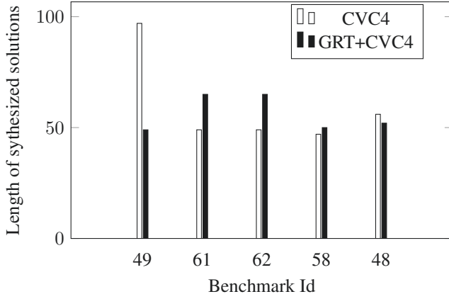
Figure 3: When the GRT+CVC4 found a different solution than CVC4, it was on average shorter than the solution found with the full grammar.
