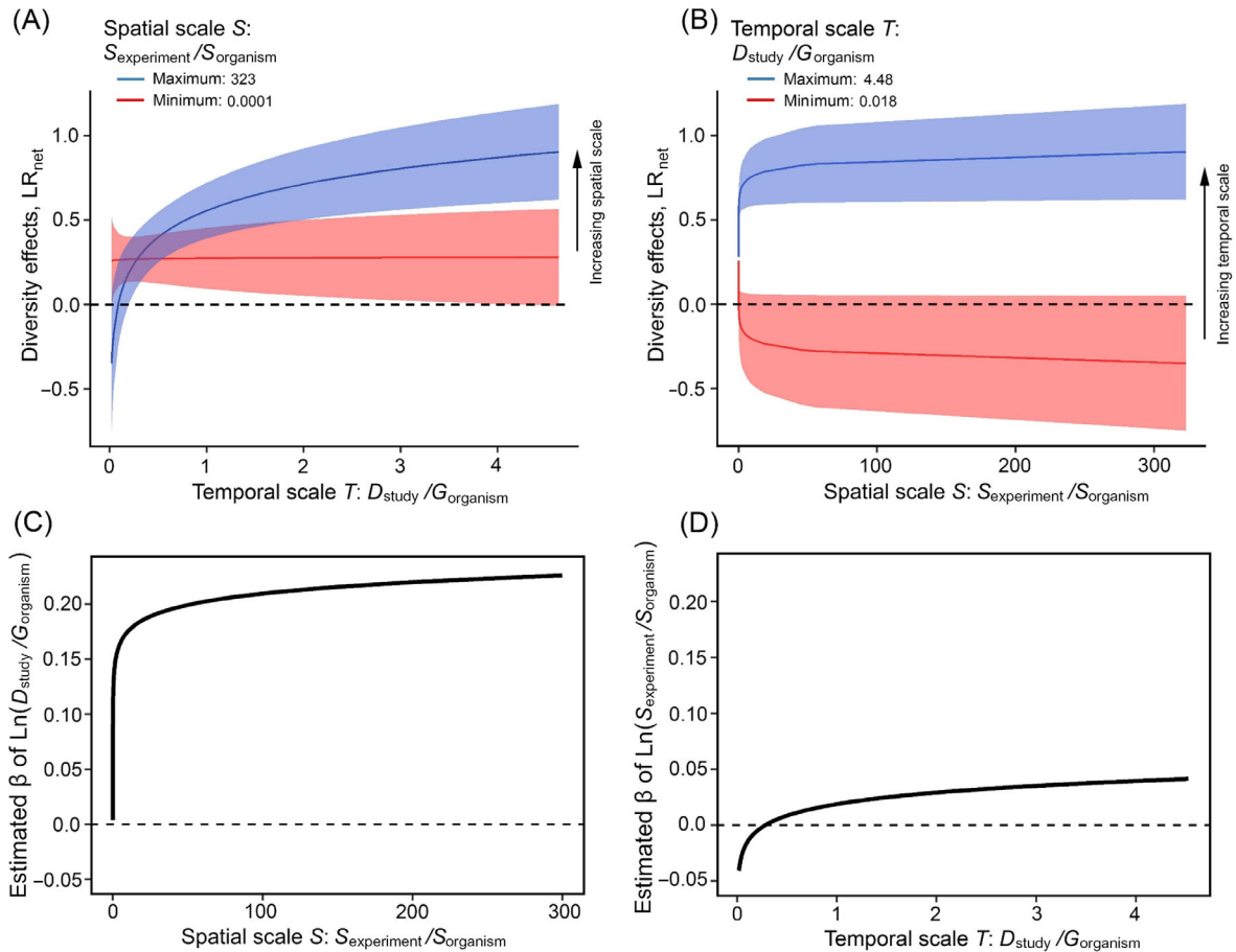
FIG. 2. Interactive effects of scales on altering plant diversity effects on biomass production: (A) how plant diversity effects, LR_{\text{net}} , vary in response to temporal scale (x-axis), whereas spatial scales are held constant at two extremes (i.e., minimum and maximum, in red and blue color, respectively); (B) how plant diversity effects, LR_{\text{net}} , vary in response to spatial scale (y-axis), whereas temporal scales are held constant at two extremes (i.e., minimum and maximum, in red and blue, respectively); (C) estimated slope \beta of temporal scales (i.e., effects of temporal scales on LR_{\text{net}} ) in responses to spatial scales; (D) estimated slope \beta of spatial scales (i.e., effects of spatial scales on LR_{\text{net}} ) in responses to temporal scales.
