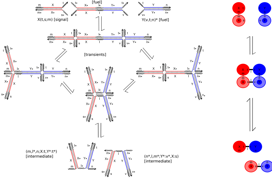
Figure 2 A cooperative 4-way branch migration mechanism. Initial X and Y complexes combine with a gate that matches their open toehold combinations, producing two 3-stranded complexes each with one of the strands of X and one of the strands of Y . These complexes can recombine with each other or with the corresponding products of a similar reaction, which in the latter case will produce X and Y complexes with different toehold combinations. On the right, this reaction is shown in abstracted form. The cooperative 4-way CRN is based on groups of four of these reactions, two in the reverse of the direction shown, where in the reverse reactions each product of one forward reaction interacts with the corresponding product of the other forward reaction. Complexes are labeled with names in the abstract notation if applicable, and their role in the cooperative 4-way CRN implementation scheme. “Signal” and “fuel” complexes have 2 strands as desired; stable “intermediate” complexes can have any number of strands; and “transient” complexes will quickly decay to one side or the other of the reaction. The marking of X(t, s, m) as signal and Y(v, t, n)^* as fuel is based on the CRN implementation scheme presented in Section 3, but in general the two can be any combination of signal and fuel, or could be intermediates of a more complex pathway.
