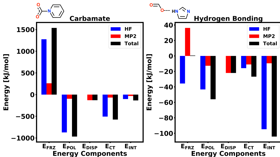
Figure 10: RMP2-EDA results (using the aug-cc-pVTZ basis) for the carbamate and hydrogen bonding motifs of \text{CO}_2^{\bullet-} , separated into HF and MP2 contributions.
