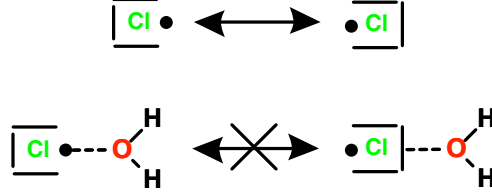
Figure 2: Illustration of the degenerate electronic configuration of the \text{Cl}^\bullet radical, which then yields distinct frozen energies for the \text{Cl}^\bullet \cdots \text{H}_2\text{O} complex depending on the initial orientation of the \text{Cl}^\bullet spin density.
