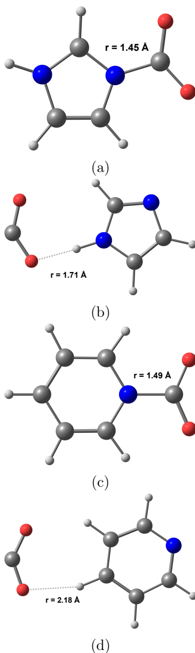
Figure 9: Geometries of the four possible isomers using both binding motifs for the reaction of a \text{CO}_2^{\bullet} with nitrogen heterocycles: (a) carbamate Im- \text{CO}_2^{\bullet} ; (b) hydrogen-bonded Im- \text{CO}_2^{\bullet} ; (c) carbamate Py- \text{CO}_2^{\bullet} ; (d) hydrogen-bonded Py- \text{CO}_2^{\bullet} .
