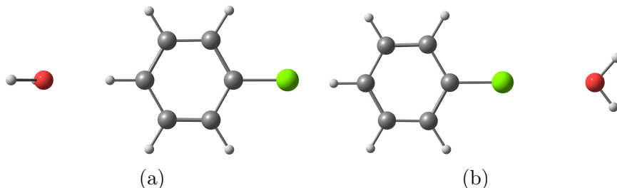
Figure 4: Optimized geometries for two isomers of the halogenated benzene radical cation–water complex: (a) the IHB structure ( r_{\text{H}\cdots\text{O}} in Å: F: 2.02, Cl: 2.04, Br: 2.05, I: 2.08); (b) the IXB structure ( r_{\text{X}\cdots\text{O}} in Å: F: 2.97, Cl: 2.78, Br: 2.78, I: 2.83).
