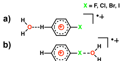
Figure 3: Two competing binding motifs for the interaction between a halogenated benzene radical cation ( \text{C}_6\text{H}_5\text{X}^{+\bullet} ) and a water molecule: (a) Ionic hydrogen bonding (IHB) and (b) ionic halogen bonding (IXB).
