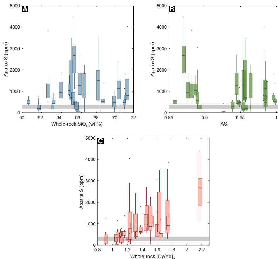
Fig. 2. Differentiation, source composition and residual garnet effects on apatite sulfur content. The data are presented as box and whisker plots of apatite S content versus pluton whole-rock \text{SiO}_2 content (A), aluminum saturation index (ASI) (B), and [\text{Dy}/\text{Yb}]_N (C). The ends of the boxes show the upper and lower quartiles, and the ends of the whiskers show the 2.5 and 97.5 percentiles. Outliers are plotted as individual points. We also measured apatite in a mafic diorite sample ( \text{SiO}_2 = 53 \text{ wt } \% ) from the Gangdese batholith, whose S contents (160 to 320 ppm) are marked by the gray bar. This shows a baseline for apatite S contents in less differentiated samples.
