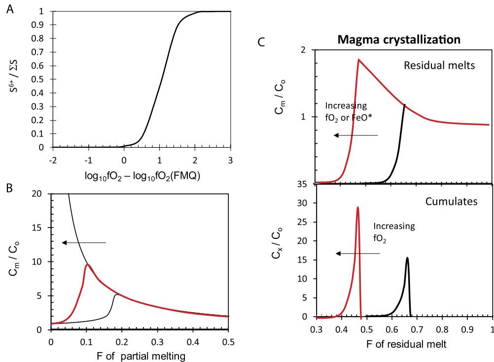
Fig. 3. Generalized behavior of S and chalcophile elements during melting and crystallization. A) Sulfur speciation in basaltic melt as a function of oxygen fugacity in \log_{10} units relative the fayalite–magnetite–quartz (FMQ) buffer (Jugo et al., 2010). B) Concentration of a chalcophile element in a primary mantle melt (equilibrium batch melt) as a function of degree of melting ( F ) of a peridotite with 200 ppm S and a chalcophile element partition coefficient between melt and sulfide of \sim 1000 . The chalcophile element is depleted in the melt before sulfide exhaustion, but after sulfide exhaustion, the chalcophile element behaves perfectly incompatibly. Point of sulfide exhaustion depends on solubility of S in the melt, which is enhanced at high fO_2 or high FeO content of melt. C) Behavior of a chalcophile element during crystallization of a magma ( F represents residual melt fraction). Top panel shows the evolution of the melt and the bottom panel represents evolution of the complementary crystal cumulates. Before sulfide saturation, the chalcophile element concentration in melt increases like an incompatible element. Once sulfide saturates, chalcophile elements are rapidly depleted from the melt. Corresponding cumulates are sulfide-free before sulfide saturation, but when sulfide saturates, cumulates experience an abrupt increase in chalcophile element concentration. Increasing fO_2 or FeO^* of the melt delays sulfide saturation. Decreasing fO_2 or FeO^* by any number of mechanisms (Jenner et al., 2010) will thus promote sulfide saturation. C_x = cumulate composition, C_m = melt composition, and C^0 = bulk composition of system. Calculations are meant to be schematic given uncertainties in sulfide solubility and S speciation as well as uncertainties in T and P of melting or crystallization. The above figures should be used only as a general guide to the behavior of S and chalcophile elements (Lee et al., 2012) as many additional factors make it challenging to develop unique models (melting degree, source composition, and effects of pressure, temperature, water and melt composition on S solubility and speciation).
