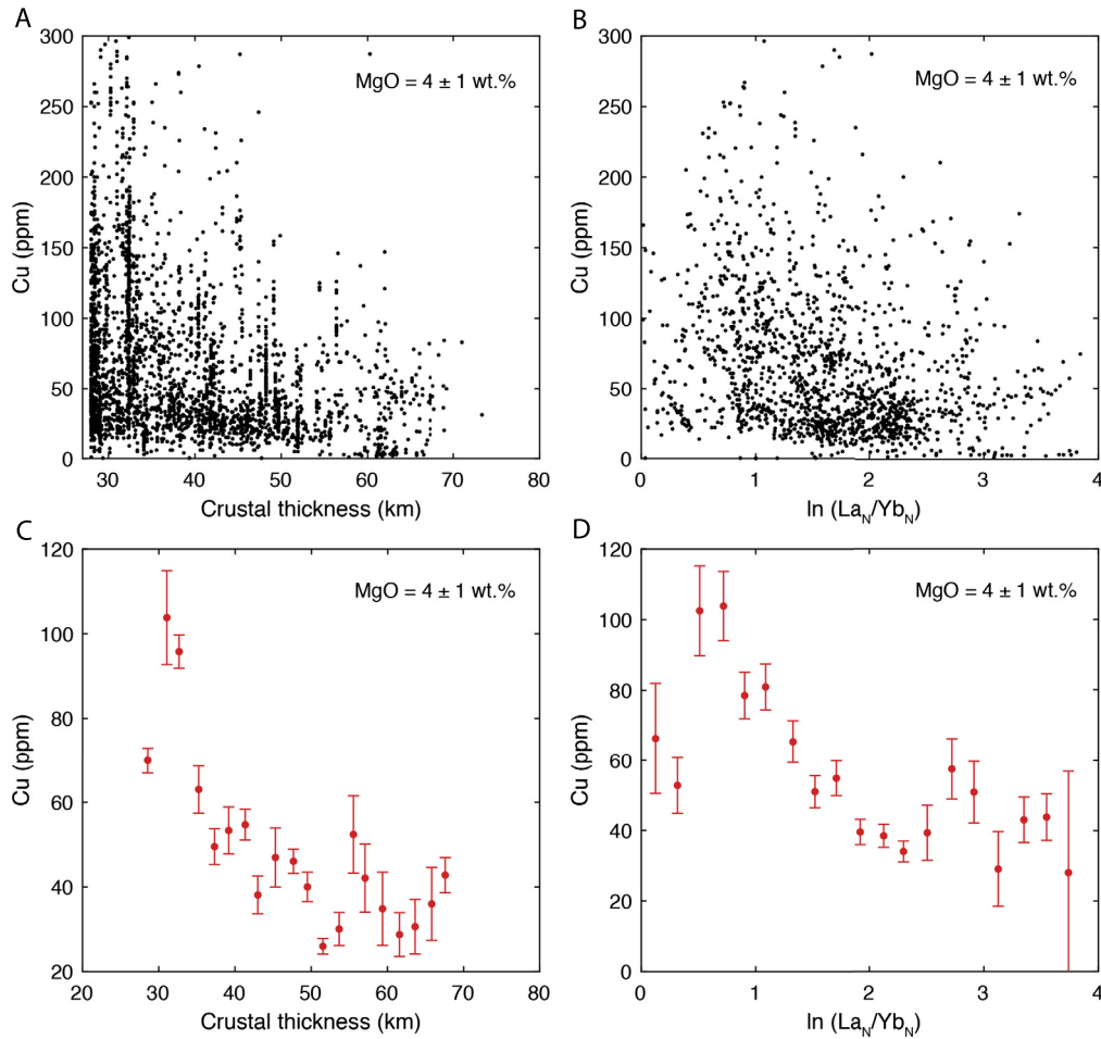
Fig. 5. Copper concentrations in modern arc magmas with 4 \pm 1 wt.% MgO as functions of crustal thickness (A) and natural logarithm of La/Yb, the latter normalized to chondrite (McDonough and Sun, 1995). (C) and (D) same as (A) and (B) respectively, but represent averages (1 standard error) of for a given crustal thickness interval. Crustal thickness is calculated from elevation assuming Airy isostasy following the methods in Lee et al. (2015) and Farner and Lee (2017). Data represent spatial averages over 1 \text{ km}^2 area to prevent sampling bias. Data are from compilation of Farner and Lee (2017) and available in Supplementary Table 1.
