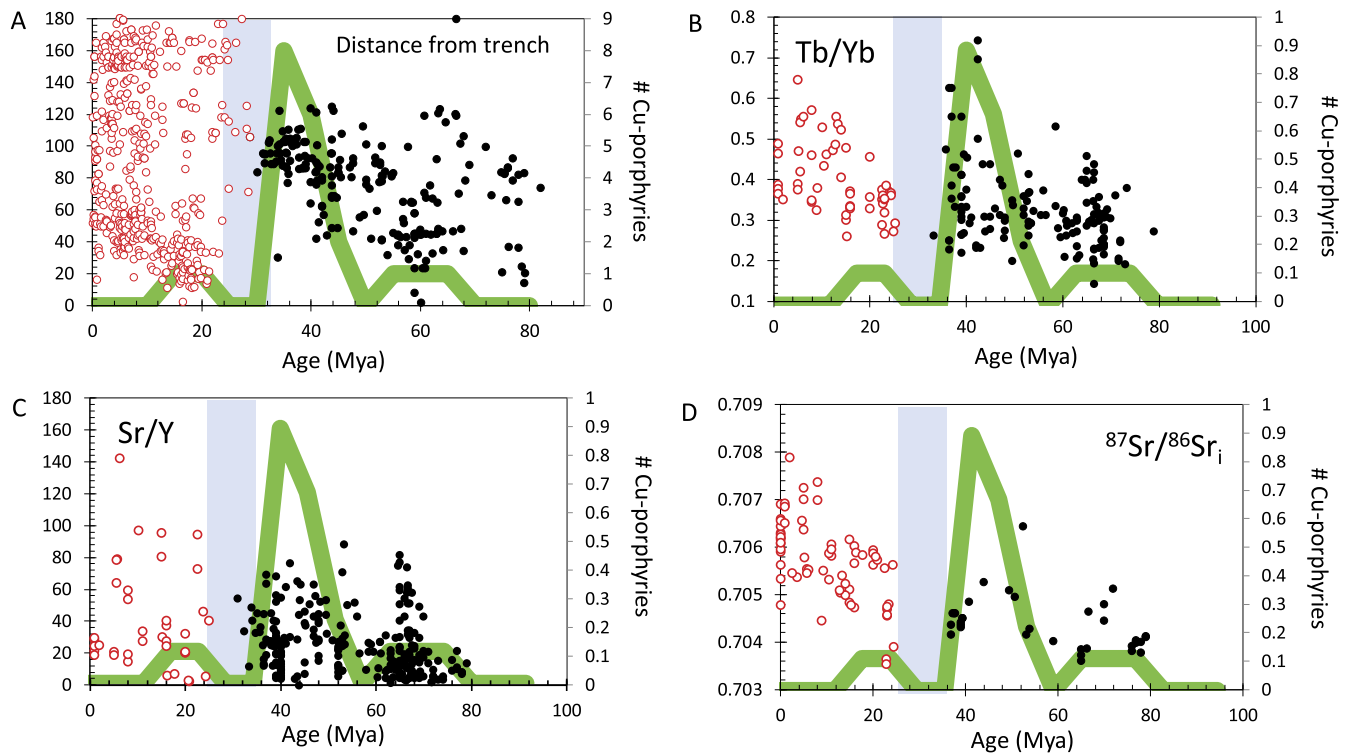
Fig. 10. Physical and geochemical evolution of arc magmas in the central Andes between 17–27 °S. A) Relative distance of arc magmas from trench (km) as a function of time (Mya = million years ago) (left hand vertical axis). Two magmatic intervals were identified (denoted by red and black) separated by a ~10 My amagmatic window (gray vertical bar). In each segment, distance is referenced to the location of the front at the beginning of each magmatic segment. Green curve represents frequency of porphyry copper deposits (right hand vertical axis). B) Tb/Yb of magmas versus age. High Tb/Yb reflects garnet fractionation. C) Sr/Y of magmas versus age. High Sr/Y reflects garnet fractionation. D) Initial ^{87}\text{Sr}/^{86}\text{Sr}_i of magmas versus age. High values indicate increased crustal assimilation. Data are from compilation by Haschke and Gunther (2003), Haschke et al. (2006) (see Supplemental Table 3).
