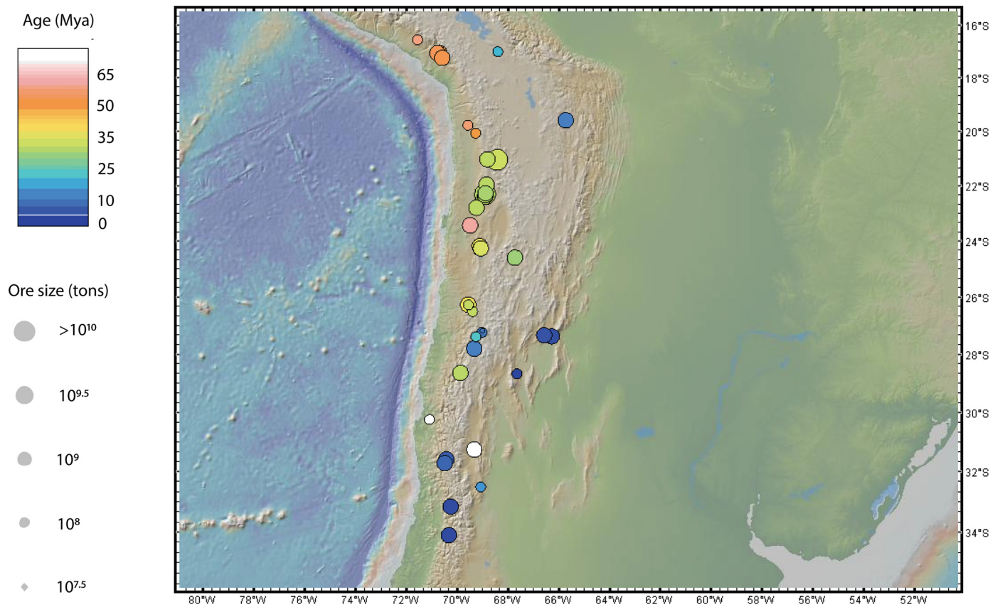
Fig. 9. PCDs in the central Andes color coded for age. Size of circles represents total tonnage (metric tons) of Cu ore. Data from Sinclair (2007) (see Supplemental Table 2).
