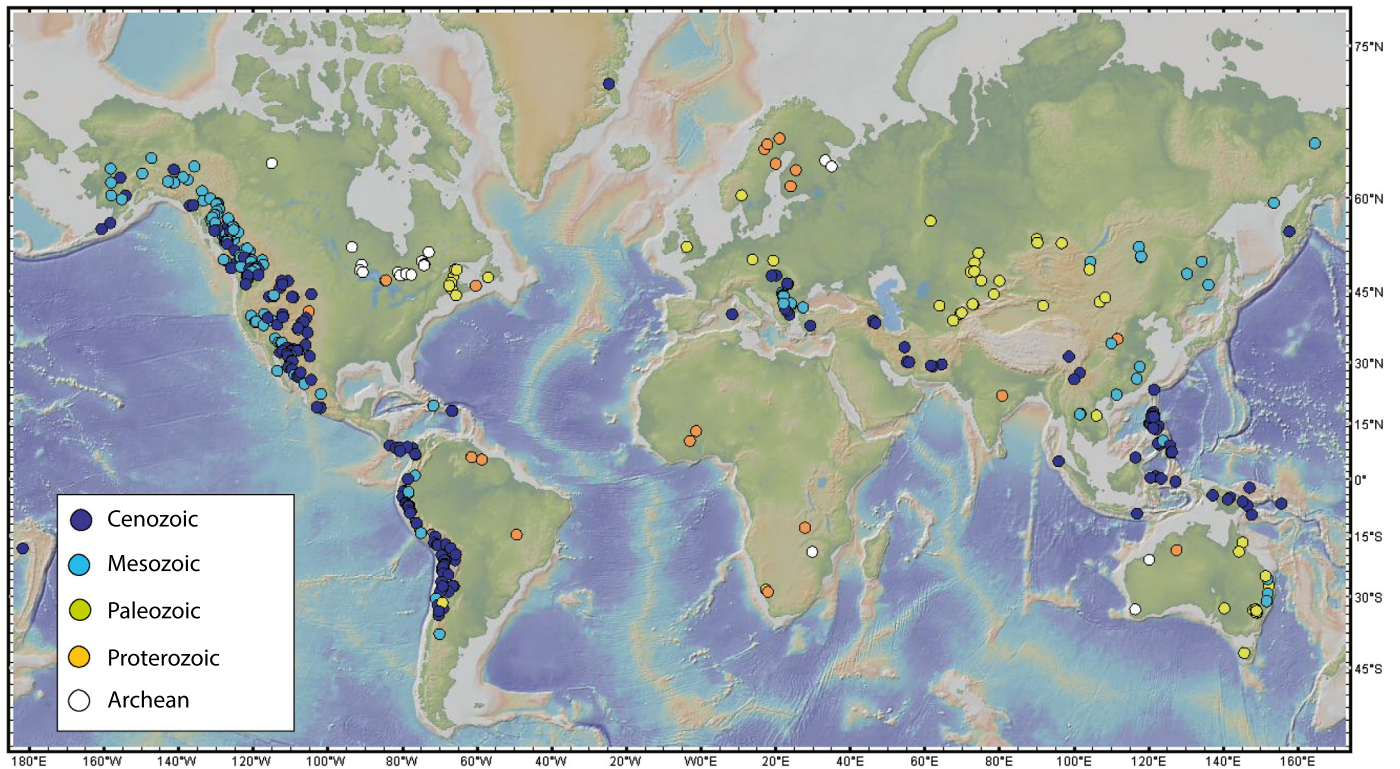
Fig. 2. Occurrence of porphyry copper deposits (PCDs) through time. All were formed in the magmatic arcs associated with subduction zones, but there is a preference for regions of thick arc crust ( > 35 km), such as continental arcs and mature island arcs. The majority are Mesozoic and Cenozoic in age due to preservation bias from the cumulative effects of erosion. Data from Sinclair (2007).
