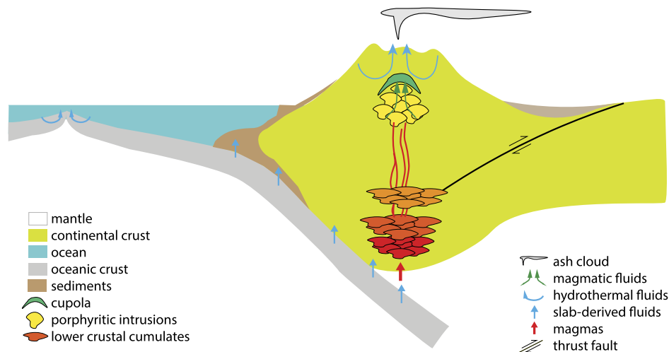
Fig. 1. Schematic of an ocean-continent subduction zone ("continental arc") denoting areas in which ore-forming elements are mobilized, transported and enriched. Here, the arc crust is thick ( > 45 km). Porphyry copper deposits (PCDs) represent shallow level intrusions (2–5 km) in the crust. Mineralization of Cu ores tend to occur at the tops of porphyry systems in cupolas. Possible regimes where Cu may be mobilized include hydrothermal circulation at mid-ocean ridge centers, dehydration or melting of the subducting slab, and late stage scavenging by magmatic fluids (green arrows). Formation of deep crustal cumulates, if sulfide-saturated, has the potential of removing and sequestering chalcophile elements like Cu deep in the crust. (For interpretation of the colors in the figure(s), the reader is referred to the web version of this article.)
