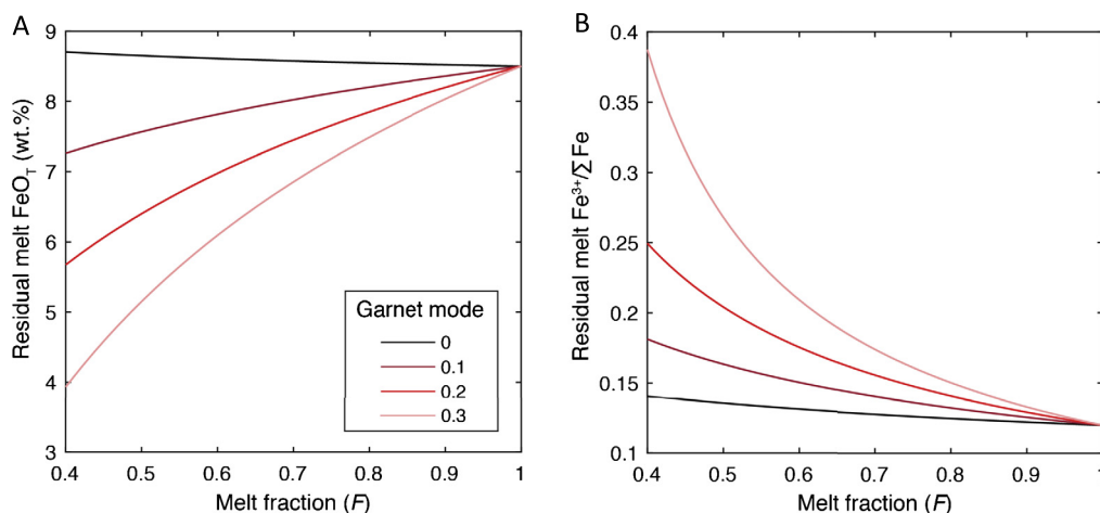
Fig. 7. Effect of garnet fractionation on the residual magma's iron content (as total \text{FeO}^* ) and the proportion of iron in the system that is ferric (molar \text{Fe}^{3+}/\Sigma\text{Fe} ). F represents residual melt fraction. Because arclogite garnets are enriched in FeO but low in ferric iron proportion ( \text{Fe}^{3+}/\Sigma\text{Fe} < 0.1 ), fractionation of garnet results in depletion in total iron ( \text{FeO}^* ) but increasing oxidation of residual iron (Tang et al., 2018; Tang et al., 2019b). Calculations were done for garnet-clinopyroxene assemblages, assuming 0–0.3 garnet modes and 0–50% total Fe depletion through garnet fractionation after 60% crystal fractionation. Non-garnet phases have a bulk D(\text{Fe}^{2+}) and D(\text{Fe}^{3+}) of 1 and 0.8, respectively. The Fe-rich arclogites in Fig. 6 typically have greater than 50% garnet.
