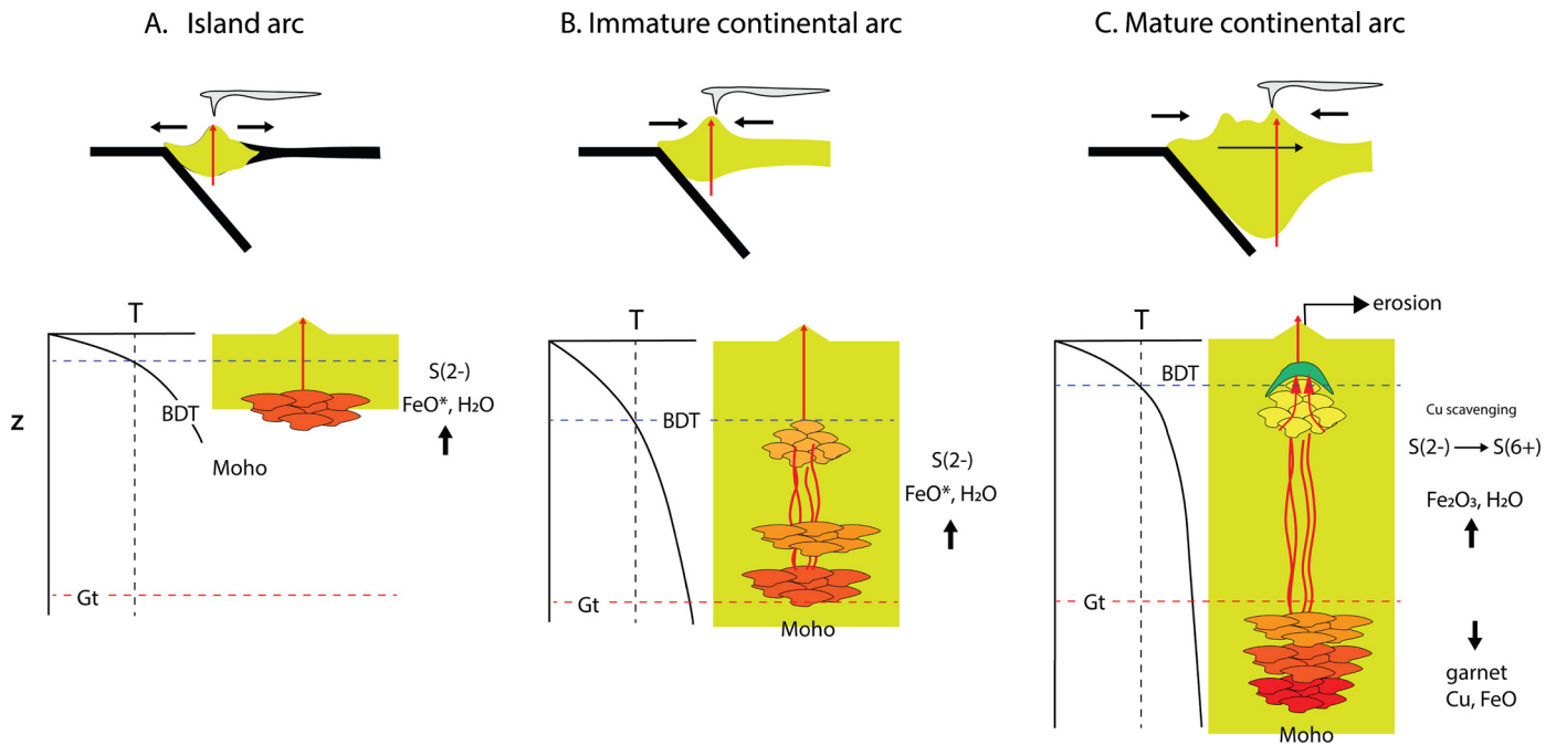
Fig. 8. Evolution of an arc as represented by schematic crustal columns and temperature–depth ( z ) profiles through the crust. A) Island arc stage when crust is thin ( < 25 km). If the upper plate is in extension, a thin arc crust is developed. Average pressures of intracrustal differentiation are low and insufficient to stabilize garnet. Because the crust is in extension, heat flow is high and geotherms are advected upwards, resulting in a shallow brittle ductile transition (BDT). Combination of stress state and shallow BDT causes residence time of magmas in the crust to be low and allows magmas to readily breach the surface and erupt. B) Immature continental arc stage (25–35 km). Upper plate is under compression, which deepens early intracrustal differentiation as well as upper crustal magmatic differentiation. Thickening also causes geotherm depression, which deepens the BDT, further frustrating eruption and development of shallow level magma bodies. C) Mature continental arc stage ( > 45 km). As arc crust becomes thicker, magmatic arc front migrates away from the trench and pressure of initial intracrustal differentiation becomes sufficient to stabilize garnet. Thermal incubation by the passage of magmas elevates geotherms, while erosion (enhanced by the high elevations), causes further shallowing of the BDT. Consequently, later stage magmas are allowed to emplace shallowly and generate porphyries. Garnet fractionation removes Fe from the residual magma, causing a decrease in S solubility, which in causes sulfide segregation and sequestration of Cu into lower crustal cumulates. Residual magmas become more oxidized, increasing Cu scavenging power of the magma. At shallow levels, degassing releases the oxidized magmatic fluids, which then migrate from the entire magma body and concentrate near the top, forming a Cu-enriched cupola. In thin arcs, residual magma does not oxidize. Cumulates are not Fe-enriched.
