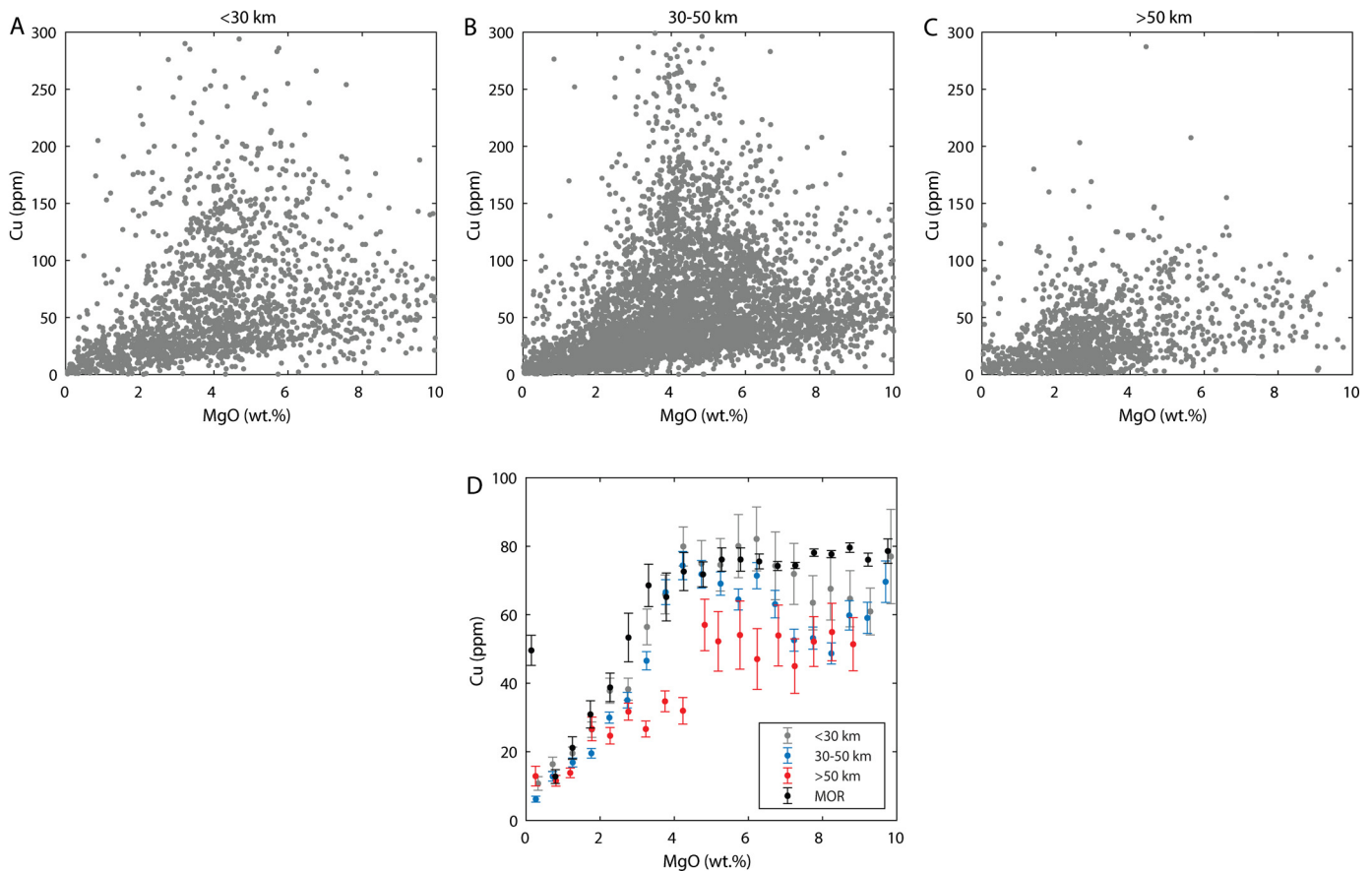
Fig. 4. Copper concentrations as a function of MgO in modern arcs built on thin (< 30 km, A), normal (30–50 km, B) and thick (> 50 km, C) crust. Island arcs are thin and continental arcs are generally thick. The arc samples examined here are volcanic rocks of Pleistocene to Holocene ages. Shown in D are MgO-binned (bin size = 0.5 wt.%) average Cu concentrations in mid ocean ridge settings (MOR) and arcs of thin, normal and thick crust. Arc data are from Farner and Lee (2017) and MOR data are from Jenner et al., (2010).
