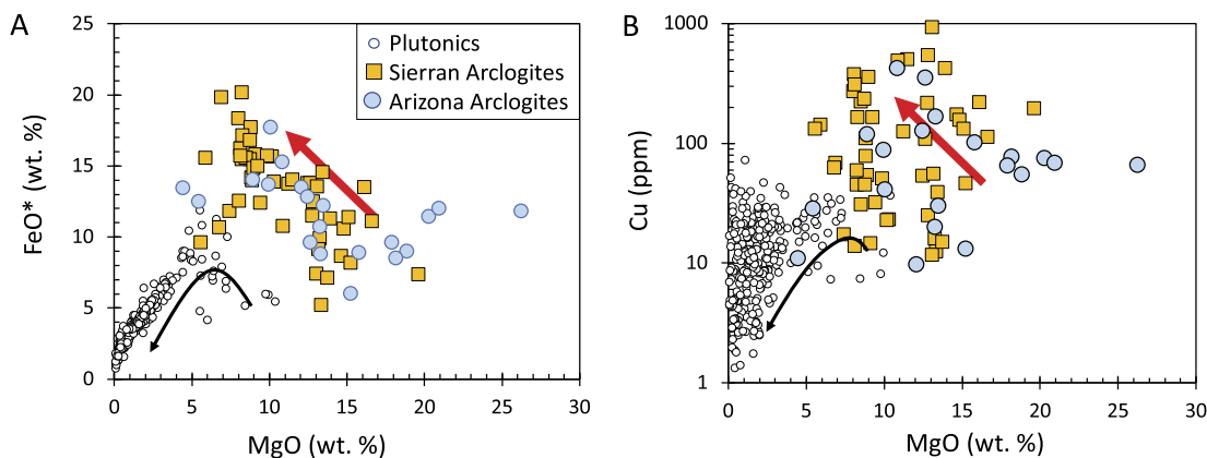
Fig. 6. \text{FeO}^* (as total Fe) and Cu in Cretaceous–Paleogene arclogite xenoliths sampled from beneath the Sierra Nevada batholith (Lee et al., 2006, 2012) and in western Arizona (Chin et al., 2018; Erdman et al., 2016) compared to Cretaceous continental arc plutonic rock compositions (as represented by the Peninsular Ranges batholith in southern California Lee et al., 2007). Note that FeO- and Cu-depleted nature of evolved plutonic rocks can be explained by eventual fractionation of FeO- and Cu-rich arclogites. Arrows represent differentiation trends (black = magma; red = arclogite cumulates).
