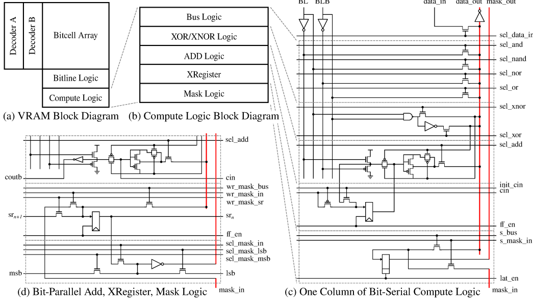
Figure 1. VRAM Circuits – High-level block diagram of VRAM microarchitecture showing a column slice of circuit-level details of all the different logic blocks of both VRAM flavors. BP-VRAM shares many logic blocks implementation with BS-VRAM, shown in (c), and only differ in three blocks that are shown in (d). The boxed logic blocks are explained in section II from top to bottom. The blocks are: bus logic, XOR/XNOR logic, ADD logic, XRegister, and mask logic.
