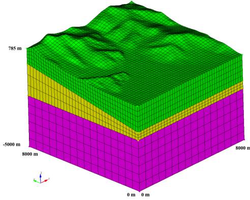
Fig. 6. Realistic topography modeling with the hp-adaptivity technique. The top surface is with free boundary condition; whereas all other boundaries are with perfectly matched layers. A second-order mesh mapping technique is utilized to capture the variance of the ground. The two heterogeneous interfaces are on a plane, determined by three vertices \{(8000, 0, -1523.14), (0, 0, -1523.14), (0, 8000, -112.52)\} m, and another plane Z = -2000 m.
