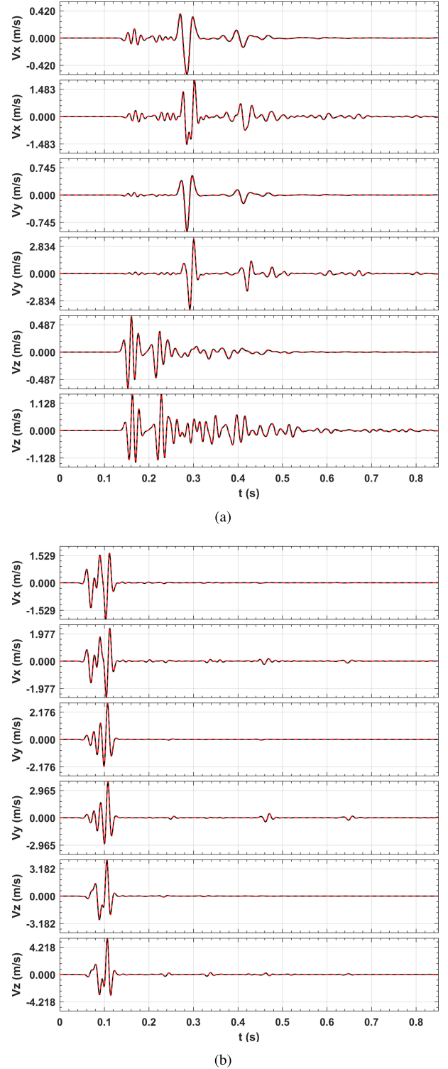
Fig. 5. Waveform comparisons of the solid particle velocity for the receivers at (a) (100, 100, -70) and (b) (100, 100, -560) in the first and fifth layers, respectively. Note that the black solid lines come from the FDTD algorithm, while the red dashed from the DG; the odd rows correspond to viscous poroelastic model, while the even for the purely poroelastic.
