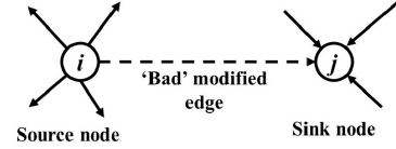
Fig. 1: An example of a minimally-influential edge with c_{ij} = T-1 .
