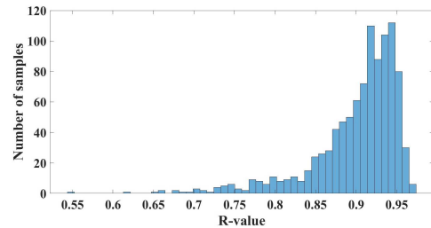
Fig. 2: Histogram of the correlation coefficient ( R -value) between the values of \{c_{ij}\}_{i,j} and \{\frac{\partial \text{tr}(\mathcal{W}_A)}{\partial a_{ji}}\}_{i,j} for 10^3 random networks with 25 node, 8 inputs and 0.2 as edge existence probability, suggesting that the former can be used as a proxy for the latter.
