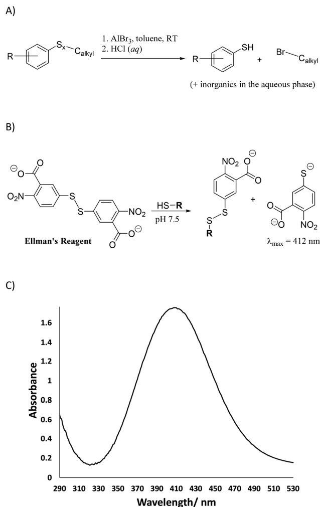
Scheme 4 (A) The reaction of AlBr 3 with organosulfur compounds. (B) The reaction of Ellman's reagent with aryl thiols to give a colorimetric response. (C) UV spectrum from Ellman's analysis of products resulting from depolymerization of XS81 by reaction with AlBr 3 .
