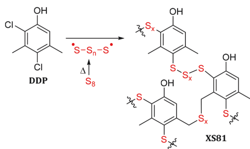
Scheme 3 Preparation of XS81 by RASP. Only the covalently-incorporated sulfur is shown in this structure.
