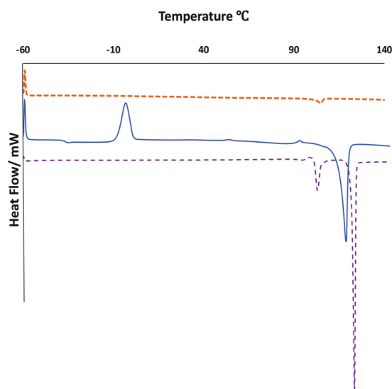
Fig. 3 DSC data analysis of sulfur (lower dashed line), XS81 (solid line), and CS 2 -insoluble fraction of XS81 (upper dashed line).
