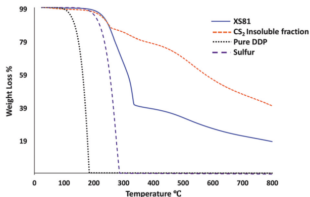
Fig. 2 TGA traces for sulfur, pure DDP monomer, XS81, and CS 2 -insoluble fraction of XS81.
