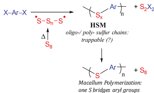
Scheme 2 Formation of S– C_{\text{aryl}} bonds by reaction of sulfur with an aryl halide in Macallum polymerization or RASP.
