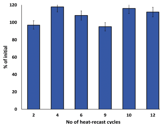
Fig. 4 The mechanical strength of XS81 is retained over at least a dozen break-melt-cast reprocessing cycles.
