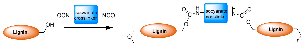
Scheme 1. Prototype reaction showing urethane bridge formation with lignin and isocyanate crosslinkers.
