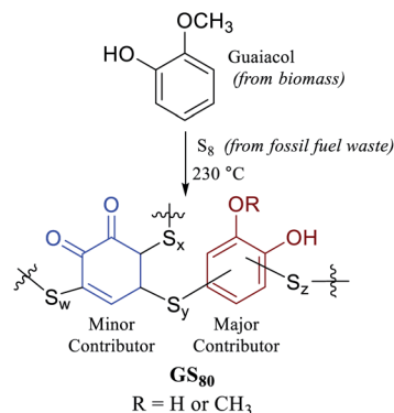
Scheme 2 Preparation of GS 80 .
