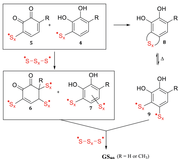
Scheme 4 Formation of GS_{80} from compounds 4, 5 and 8.
