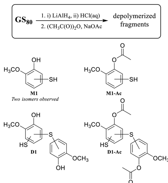
Chart 2 Depolymerization products from GS_{80} observed by GC-MS. Mass spectra for these species are provided in ESI Fig. S5–S8.†
