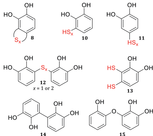
Chart 1 Products previously observed from reaction of polymeric sulfur radicals and o -quinone.
