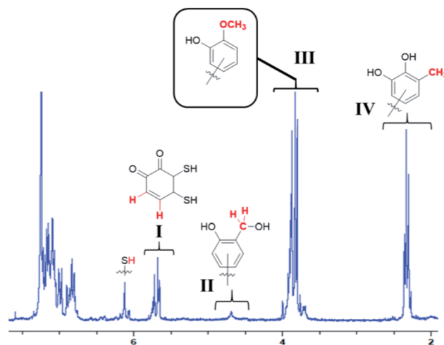
Fig. 1 Proton NMR spectroscopic analysis of GS 80 depolymerization products. Resonance groups are attributed to the red-highlighted protons within each attendant structure.
