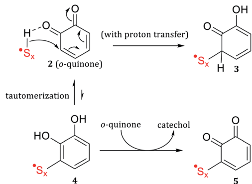
Scheme 3 Reaction of o -quinone with sulfur radicals.
