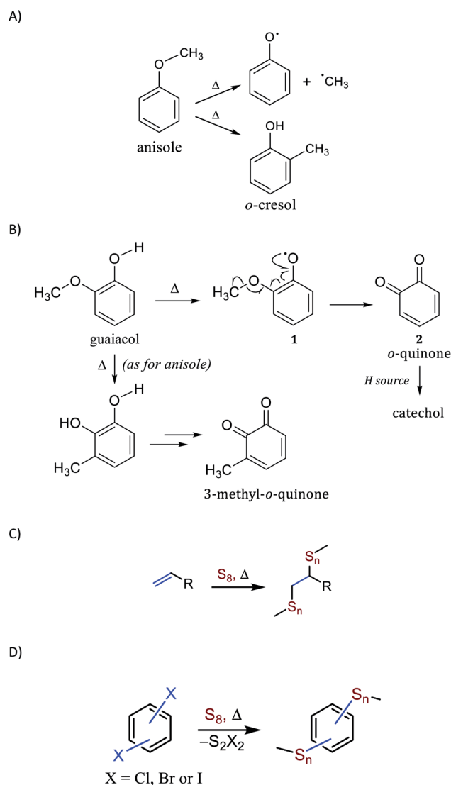
Scheme 1 Established thermal decomposition of anisole (A) and guaiacol (B) and established inverse vulcanization (C) and RASP (D) routes to HSMs.
