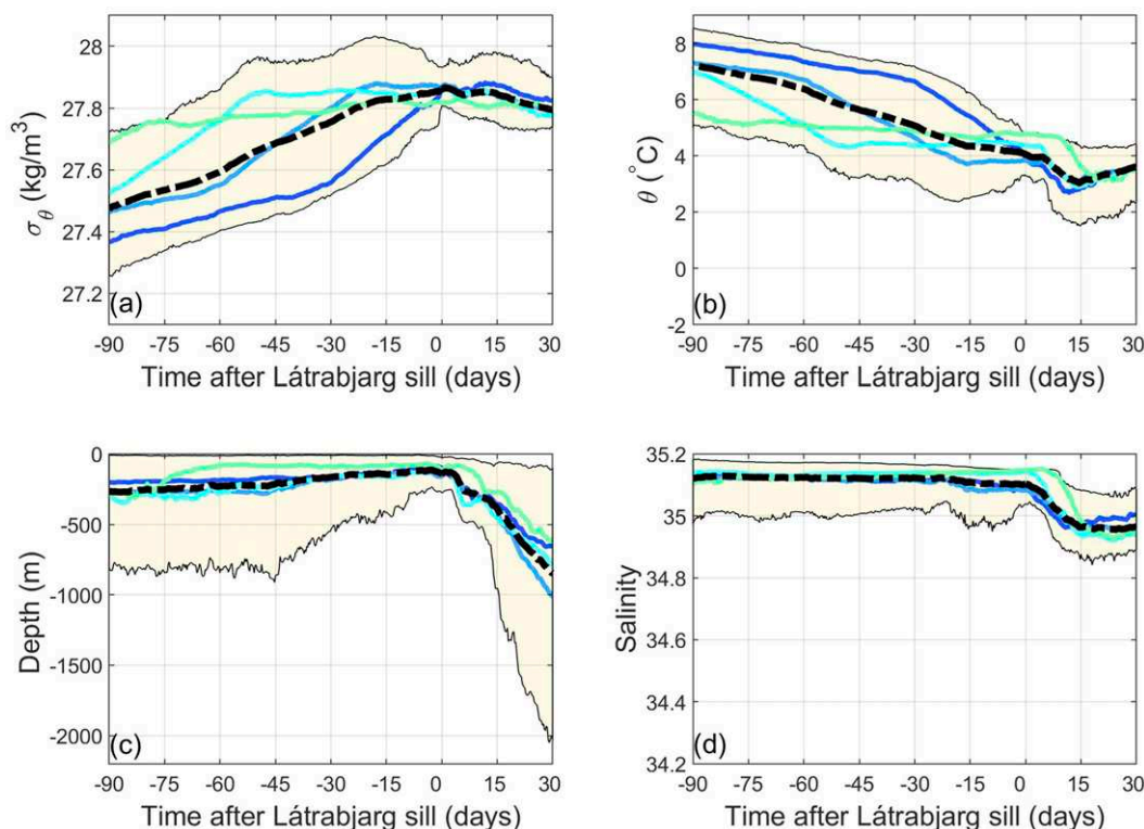
FIG. 12. As in Fig. 10, but for the DSO particles in the ISh subset. Note that the particles in this subset are only present in ensemble members III–VI.
