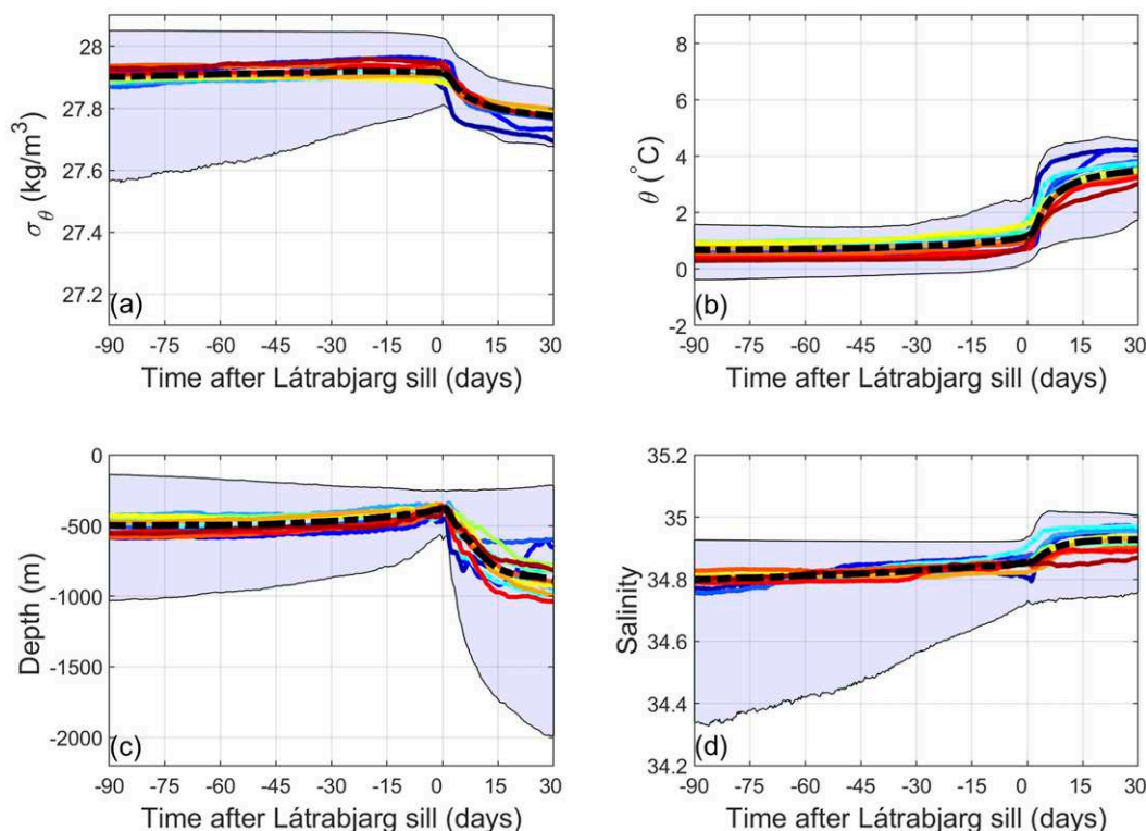
FIG. 10. The temporal evolution of (a) potential density, (b) potential temperature, (c) depth, and (d) salinity of the DSO particles in the N subset color coded by ensemble member (see Fig. 6a). The shading in each subplot marks the 5th and 95th percentiles of the DSO particle properties over all ensemble members. The individual colored solid lines show the mean properties for each ensemble member (consistent with the color codes in Fig. 6a). The black dash-dotted lines show the mean properties over all ensemble members. The abscissa shows the time line for the particles from the origin moving toward the Látrabjarg sill section (days 0) and after crossing it.
